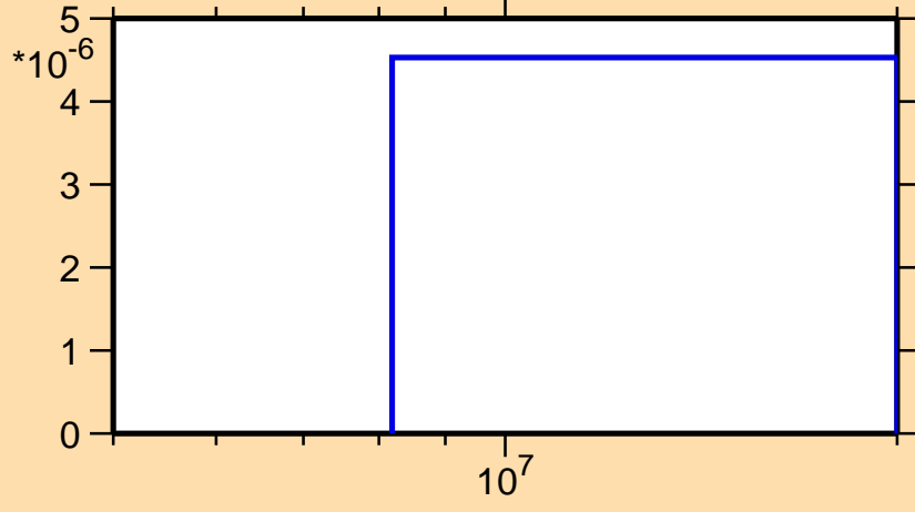
\sigma vs. E for ^{205}\text{Tl}(n,n\alpha)
