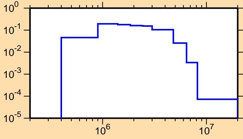
\sigma vs. E for ^{206}\text{Tl}(n,n_3)
