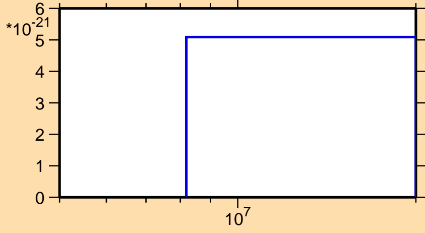
\sigma vs. E for ^{206}\text{Tl} (mt 11)
