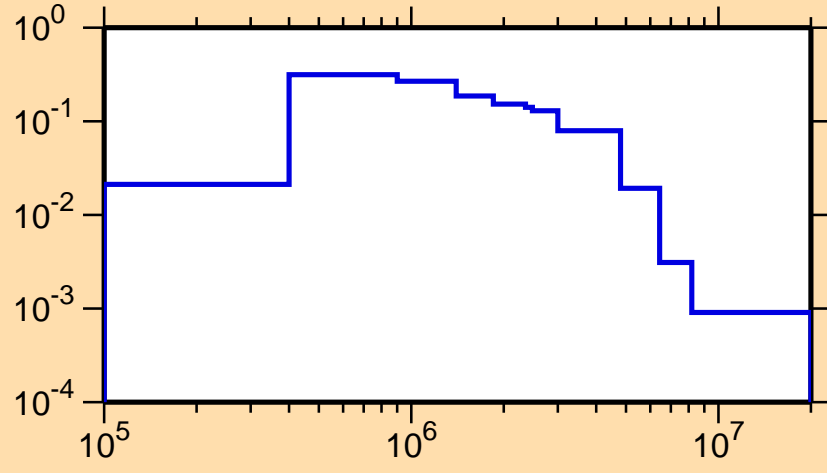
\sigma vs. E for ^{206}\text{Tl}(n,n_2)
