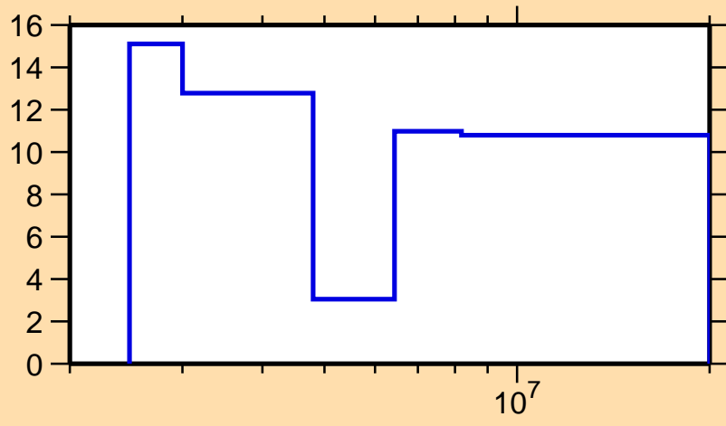
\Delta\sigma/\sigma vs. E for ^{206}\text{Tl}(n,n\text{cont.})
