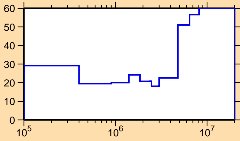
\Delta\sigma/\sigma vs. E for ^{206}\text{Tl}(n,n_1)
