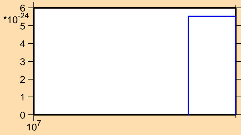
\sigma vs. E for ^{207}\text{Tl} (mt 42)
