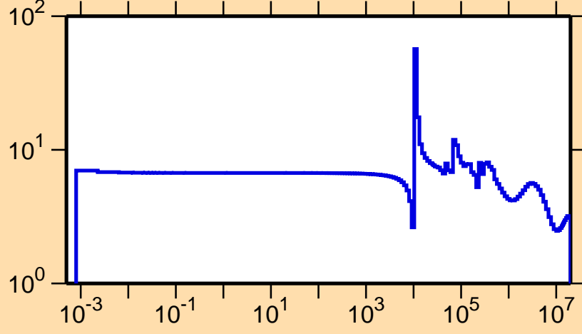
\sigma vs. E for ^{207}\text{Tl}(n,\text{el.})
