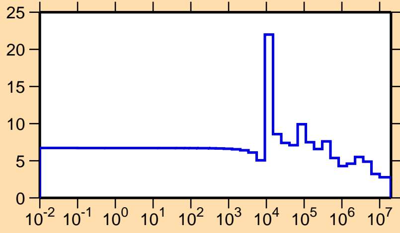
\sigma vs. E for ^{207}\text{Tl}(n,\text{el.})
