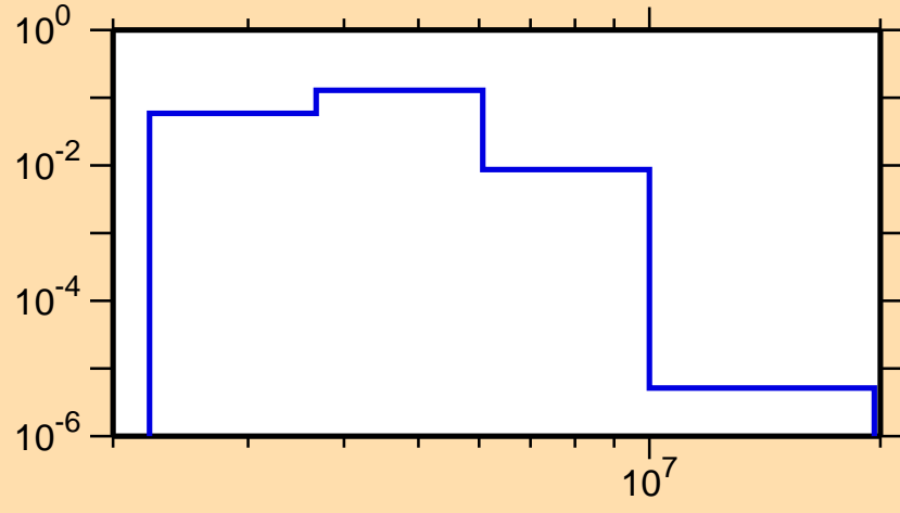
\sigma vs. E for ^{207}\text{Tl}(n,n_4)
