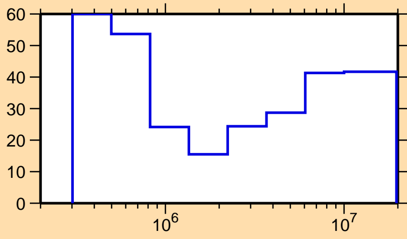
\Delta\sigma/\sigma vs. E for ^{207}\text{Tl}(n,n_1)
