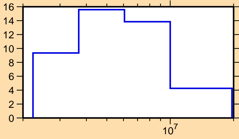
\Delta\sigma/\sigma vs. E for ^{207}\text{Tl}(n,\text{el.})
