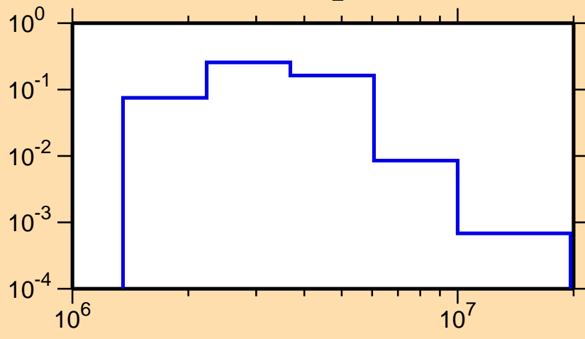
\sigma vs. E for ^{207}\text{Tl}(n,n_2)
