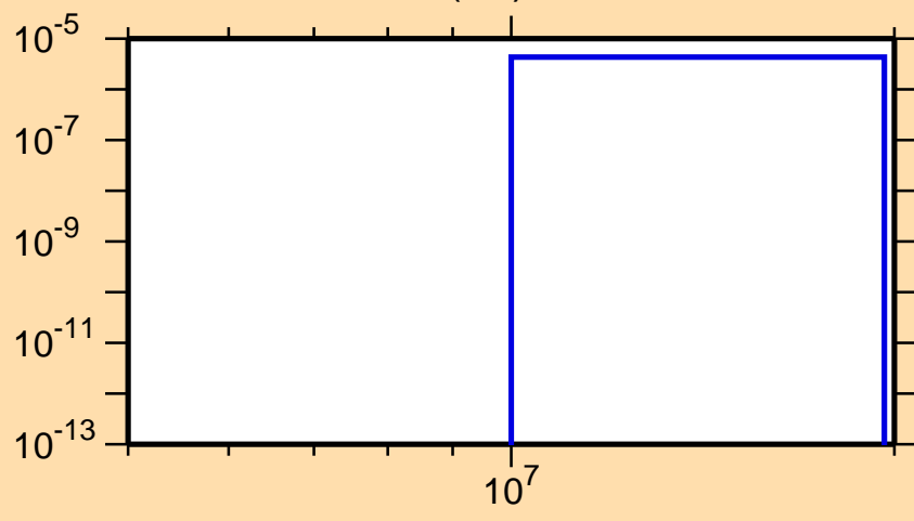
\sigma vs. E for ^{207}\text{Tl}(n,t)
