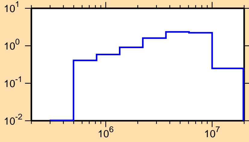
\sigma vs. E for ^{207}\text{Tl}(n,\text{inel.})
