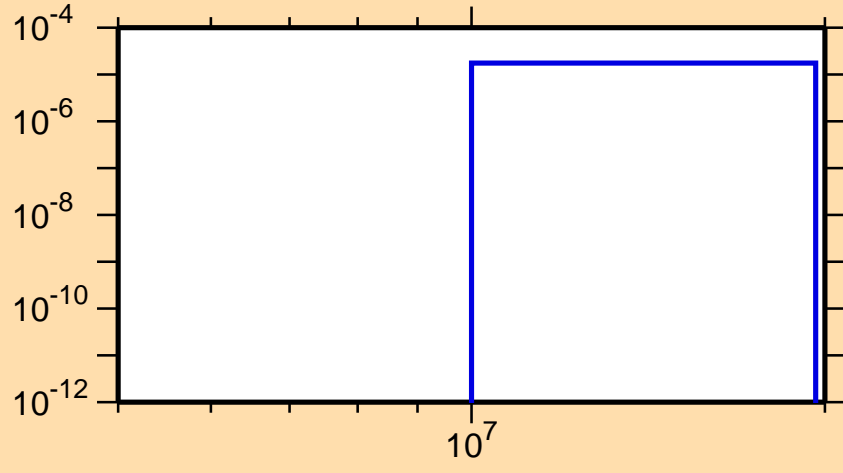
\sigma vs. E for ^{207}\text{Tl}(n,np)
