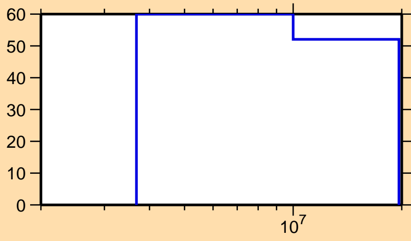
\Delta\sigma/\sigma vs. E for ^{207}\text{Tl}(n,\gamma)
