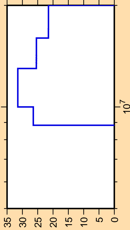
\Delta\sigma/\sigma vs. E for ^{207}\text{Tl}(n,np)
