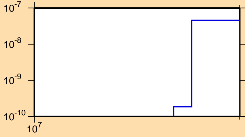
\sigma vs. E for ^{207}\text{Tl}(n,2np)
