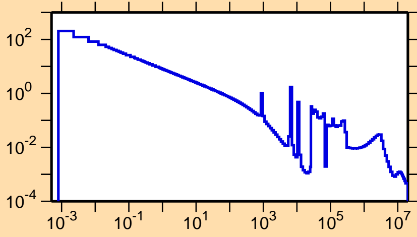
\sigma vs. E for ^{207}\text{Tl}(n,\gamma)
