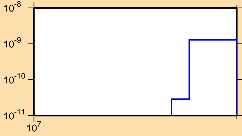
\sigma vs. E for ^{207}\text{Tl}(n,2n\alpha)
