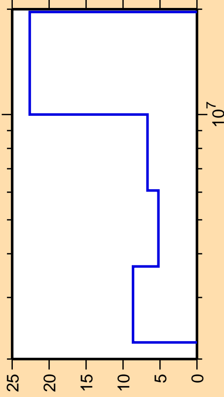
\Delta\sigma/\sigma vs. E for ^{207}\text{Tl}(n,n\text{cont.})
