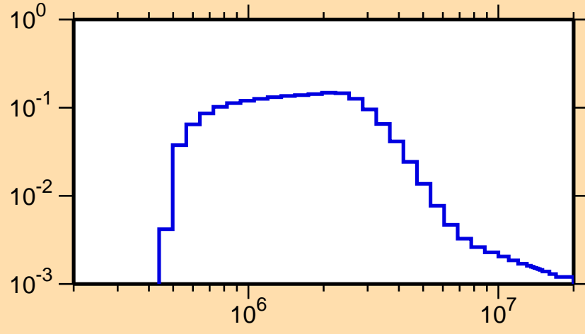
\sigma vs. E for ^{208}\text{Tl}(n,n_3)
