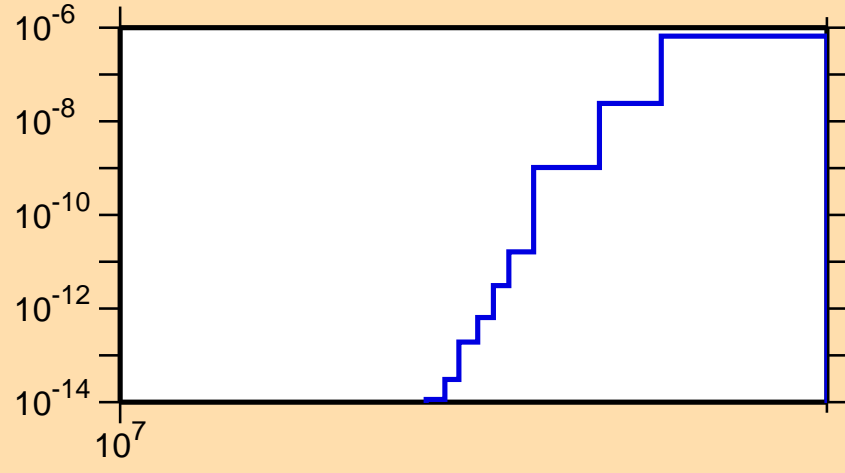
\sigma vs. E for ^{208}\text{Tl}(n,2np)
