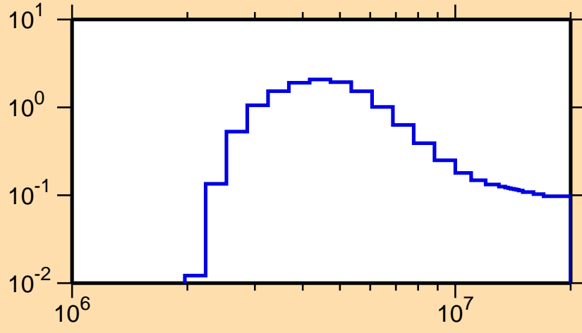
\sigma vs. E for ^{208}\text{Tl}(n,n\text{cont.})
