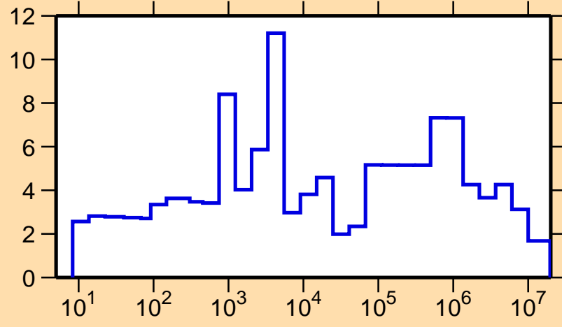
\Delta\sigma/\sigma vs. E for ^{208}\text{Tl}(n,\text{tot.})
