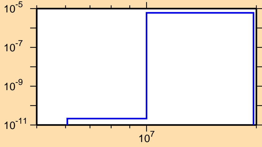
\sigma vs. E for ^{208}\text{Tl}(n,n\alpha)
