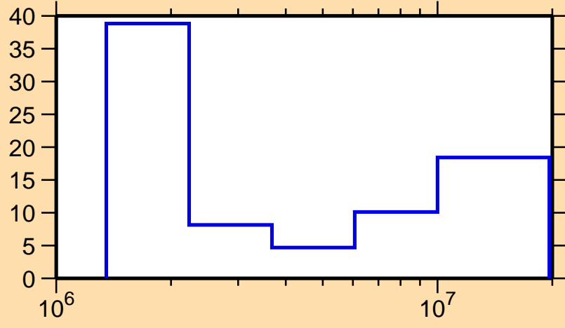
\Delta\sigma/\sigma vs. E for ^{208}\text{Tl}(n,ncont.)
