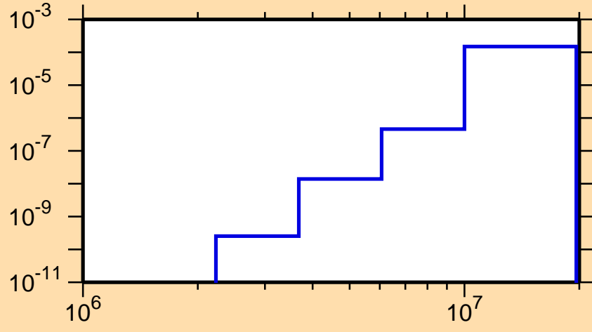
\sigma vs. E for ^{208}\text{Tl}(n,\alpha)
