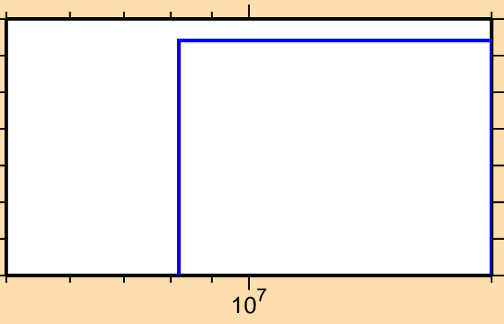
\sigma vs. E for ^{208}\text{Tl}(n,2np)
