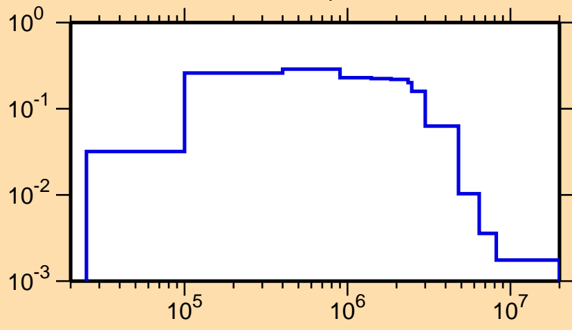
\sigma vs. E for ^{208}\text{Tl}(n,n_1)
