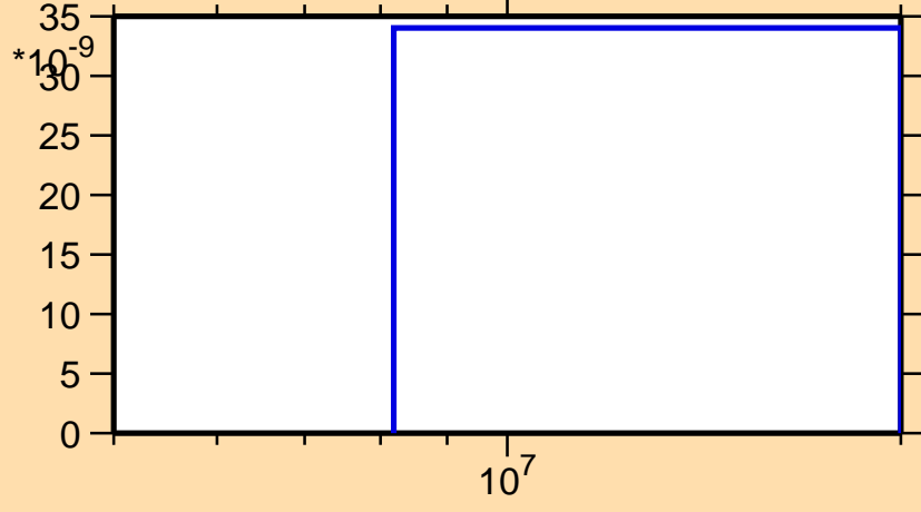
\sigma vs. E for ^{208}\text{Tl}(n,nt)
