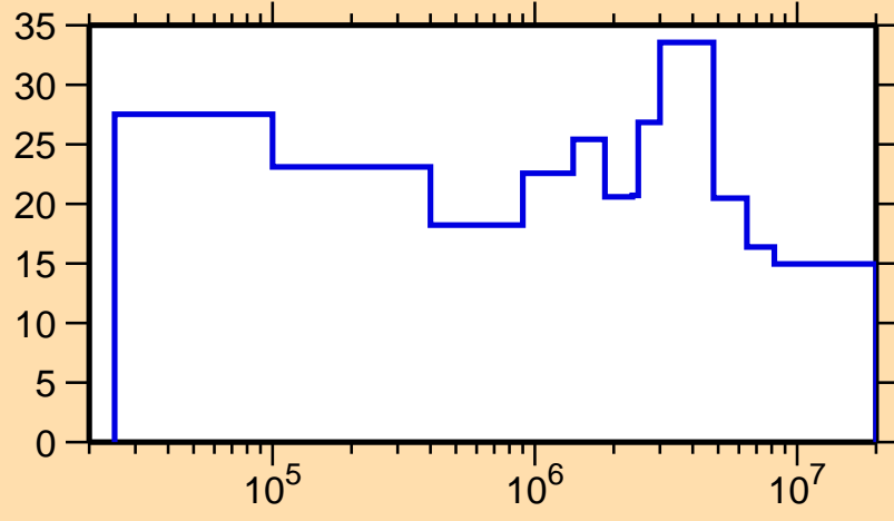
\Delta\sigma/\sigma vs. E for ^{208}\text{Tl}(n,n_1)
