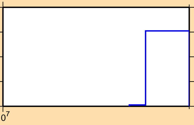
\sigma vs. E for ^{209}\text{Tl}(n,3n\alpha)
