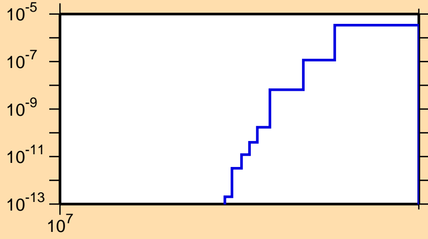
\sigma vs. E for ^{209}\text{Tl}(n,nd)
