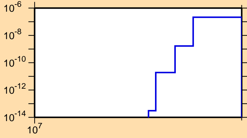
\sigma vs. E for ^{209}\text{Tl}(n,2np)
