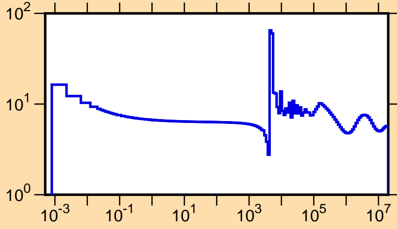
\sigma vs. E for ^{209}\text{Tl}(n,\text{tot.})
