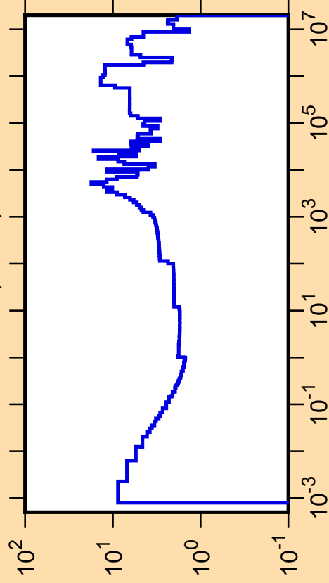
\Delta\sigma/\sigma vs. E for ^{209}\text{Tl}(n,\text{tot.})
