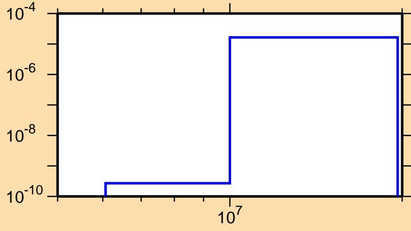
\sigma vs. E for ^{209}\text{Tl}(n,n\alpha)
