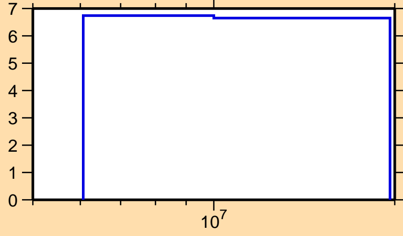
\Delta\sigma/\sigma vs. E for ^{209}\text{Tl}(n,el.)
