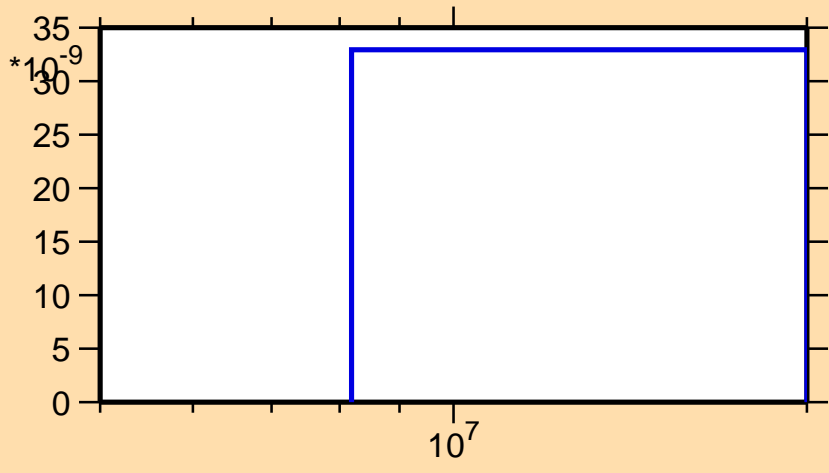
\sigma vs. E for ^{209}\text{Tl}(n,\text{nd})
