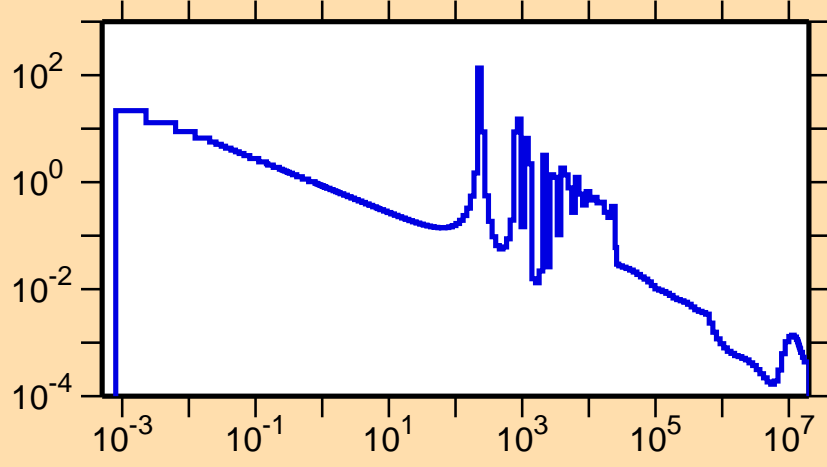
\sigma vs. E for ^{210}\text{Tl}(n,\gamma)
