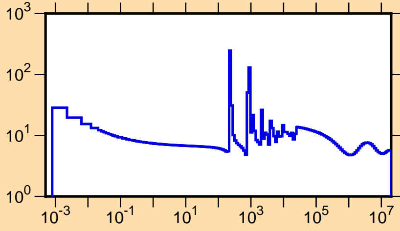
\sigma vs. E for ^{210}\text{Tl}(n,\text{tot.})
