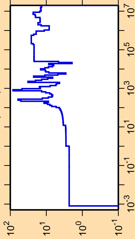
\Delta\sigma/\sigma vs. E for ^{210}\text{Tl}(n,\text{el.})
