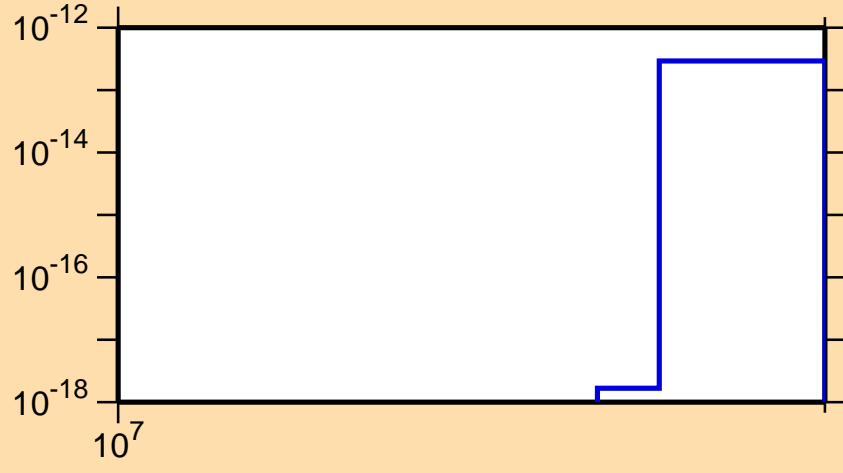
\sigma vs. E for ^{210}\text{Tl} (mt 42)
