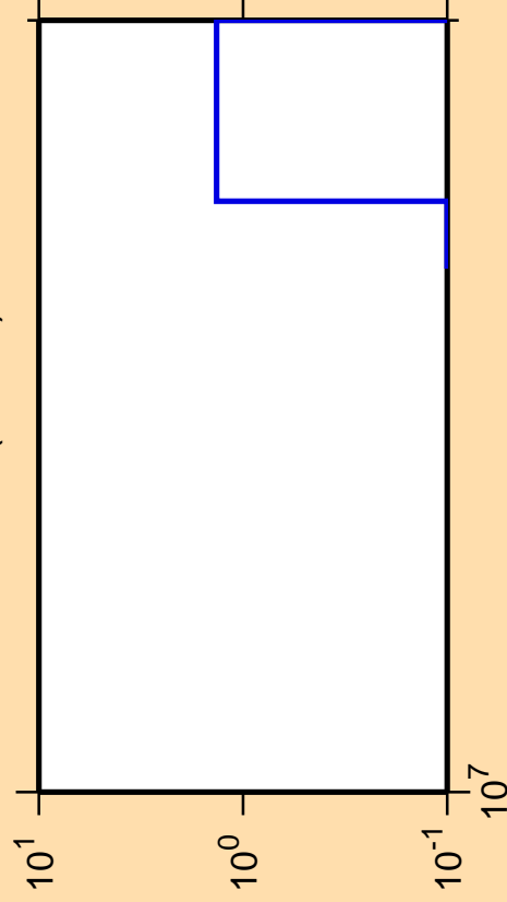
\Delta\sigma/\sigma vs. E for ^{210}\text{Tl} (mt 42)
