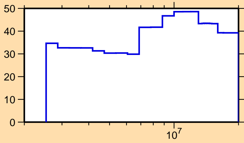
\Delta\sigma/\sigma vs. E for ^{210}\text{Tl}(n,n\text{cont.})
