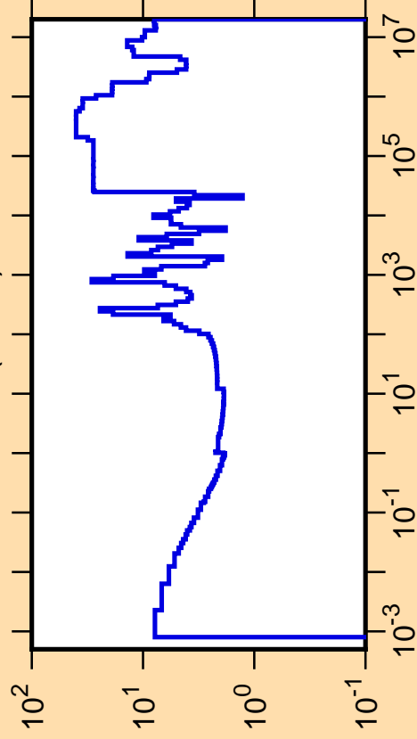
\Delta\sigma/\sigma vs. E for ^{210}\text{Tl}(n,\text{tot.})
