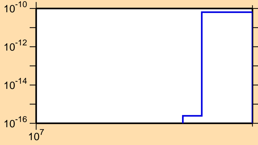
\sigma vs. E for ^{210}\text{Tl}(\text{mt 11})
