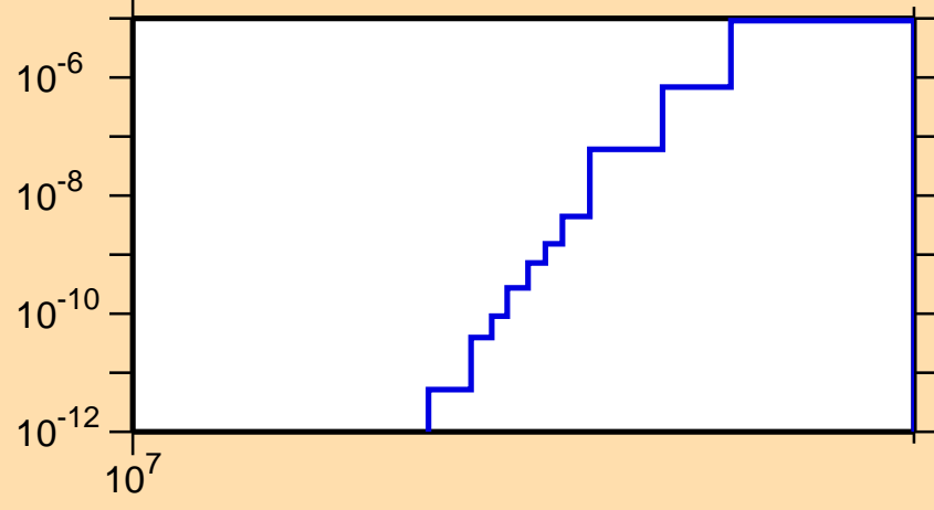
\sigma vs. E for ^{210}\text{Tl}(n,\text{nd})
