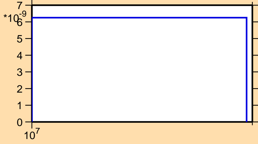
\sigma vs. E for ^{210}\text{Tl}(n,2np)
