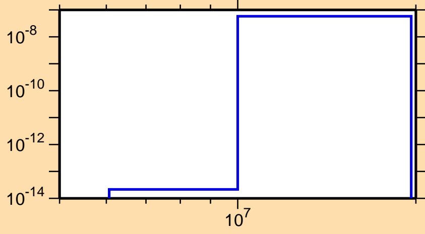
\sigma vs. E for ^{210}\text{Tl}(n,2n\alpha)
