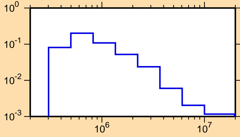
\sigma vs. E for ^{210}\text{Tl}(n,n_3)
