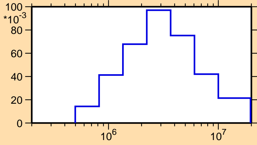
\sigma vs. E for ^{210}\text{Tl}(n,n_4)
