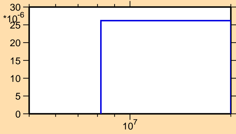
\sigma vs. E for ^{210}\text{Tl}(n,d)
