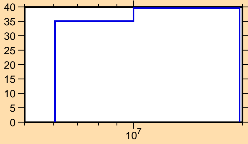
\Delta\sigma/\sigma vs. E for ^{211}\text{Tl}(n,ncont.)
