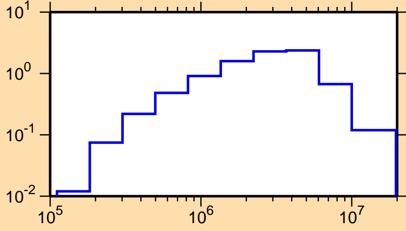
\sigma vs. E for ^{211}\text{Tl}(n,n\text{cont.})
