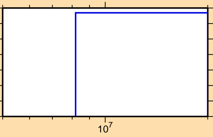
\sigma vs. E for ^{211}\text{Tl}(n,d)
