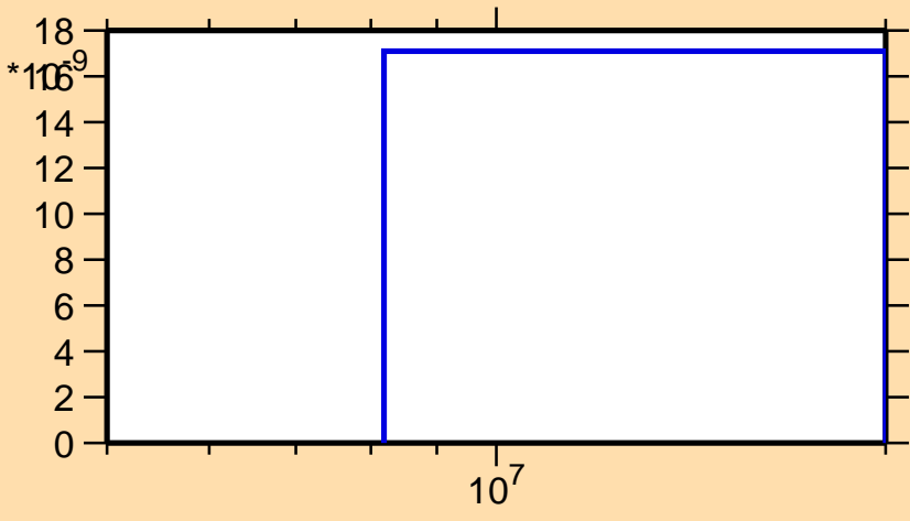
\sigma vs. E for ^{211}\text{Tl}(n,\text{nd})
