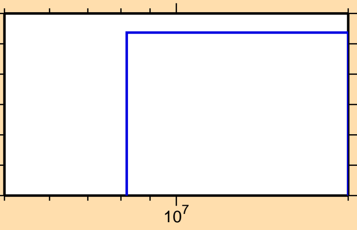
\sigma vs. E for ^{212}\text{Tl}(n,np)
