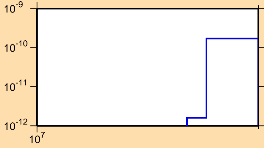
\sigma vs. E for ^{214}\text{Tl}(n,3n\alpha)
