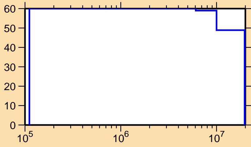
\Delta\sigma/\sigma vs. E for ^{214}\text{Tl}(n,n_1)
