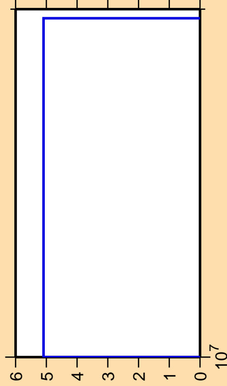
\Delta\sigma/\sigma vs. E for ^{214}\text{Tl}(n,3n\alpha)
