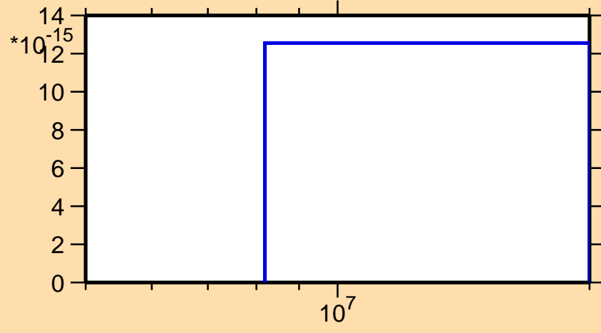
\sigma vs. E for ^{214}\text{Tl} (mt 42)
