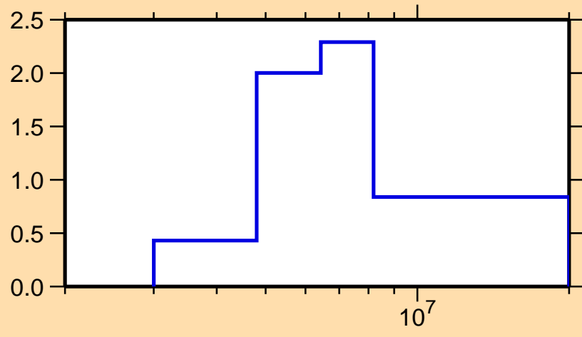
\sigma vs. E for ^{214}\text{Tl}(n,2n)
