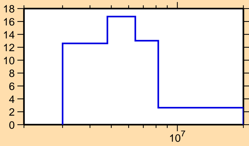
\Delta\sigma/\sigma vs. E for ^{214}\text{Tl}(n,\text{tot.})
