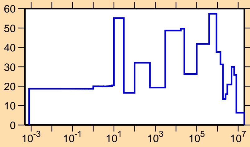
\Delta\sigma/\sigma vs. E for ^{214}\text{Tl}(n,\text{el.})
