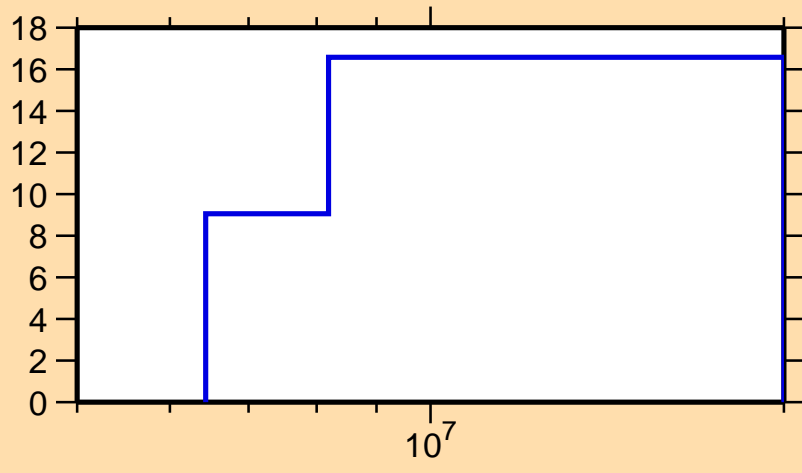
\Delta\sigma/\sigma vs. E for ^{214}\text{Tl}(n,2n)
