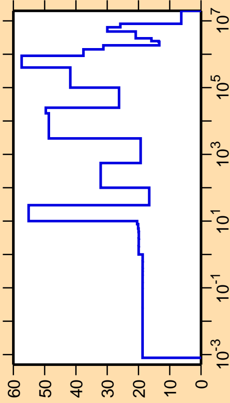
\Delta\sigma/\sigma vs. E for ^{214}\text{Tl}(n,\text{el.})
