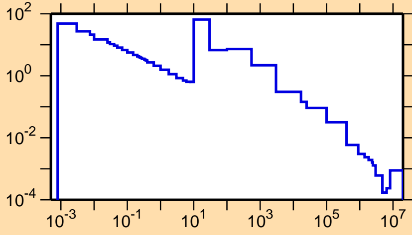
\sigma vs. E for ^{214}\text{Tl}(n,\gamma)
