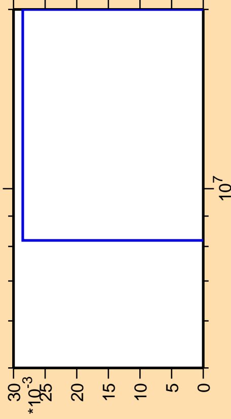
\Delta\sigma/\sigma vs. E for ^{214}\text{Tl} (mt 42)
