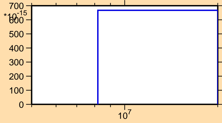
\sigma vs. E for ^{214}\text{Tl} (mt 11)
