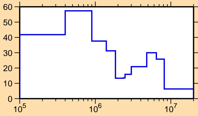
\Delta\sigma/\sigma vs. E for ^{214}\text{Tl}(n, el.)
