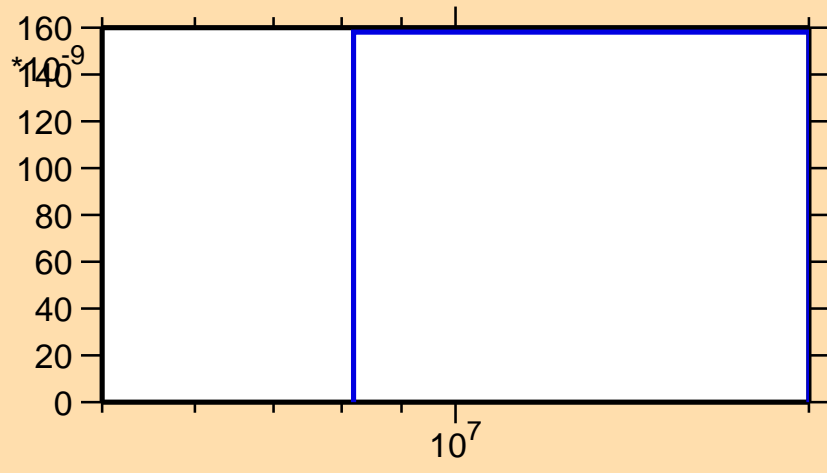
\sigma vs. E for ^{214}\text{Tl}(n,nd)
