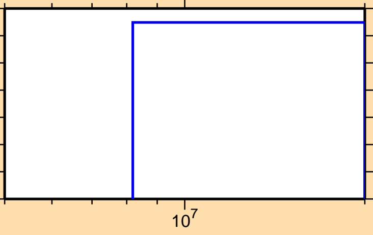
\sigma vs. E for ^{214}\text{Tl}(n,np)
