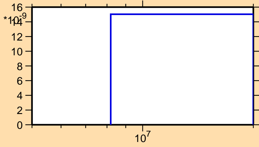
\sigma vs. E for ^{214}\text{Tl}(n,2n\alpha)
