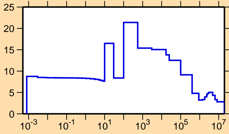
\sigma vs. E for ^{214}\text{Tl}(n,\text{el.})
