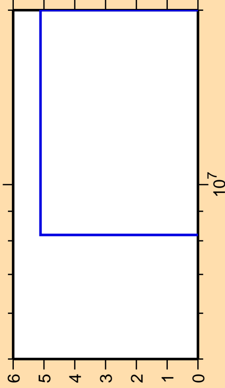
\Delta\sigma/\sigma vs. E for ^{214}\text{Tl} (mt 11)
