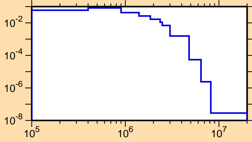
\sigma vs. E for ^{214}\text{Tl}(n,n_1)
