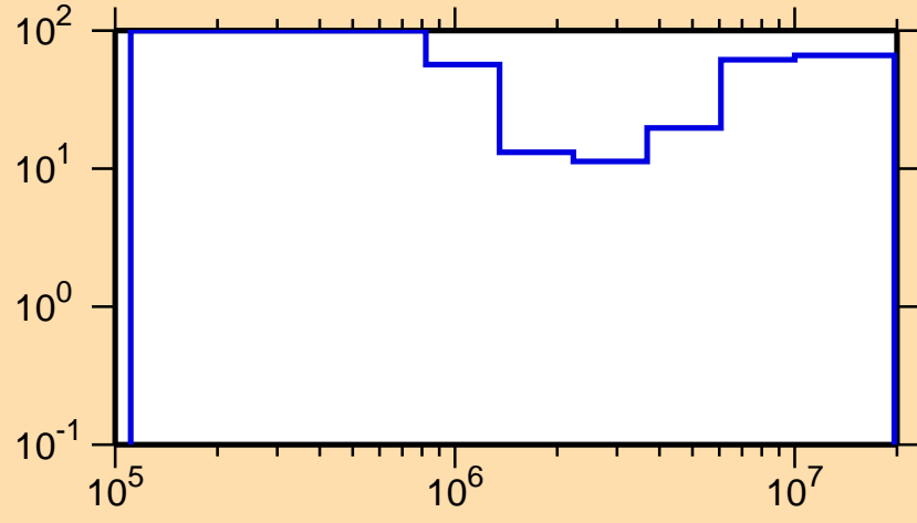
\Delta\sigma/\sigma vs. E for ^{215}\text{Tl}(n,ncont.)
