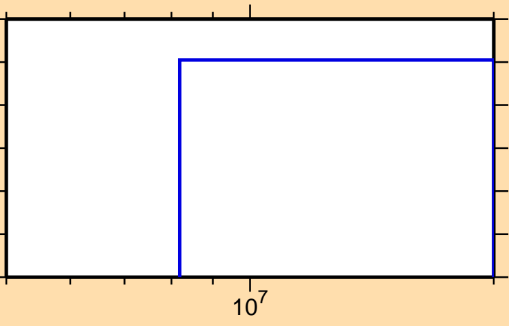
\sigma vs. E for ^{215}\text{Tl}(n,\text{nd})
