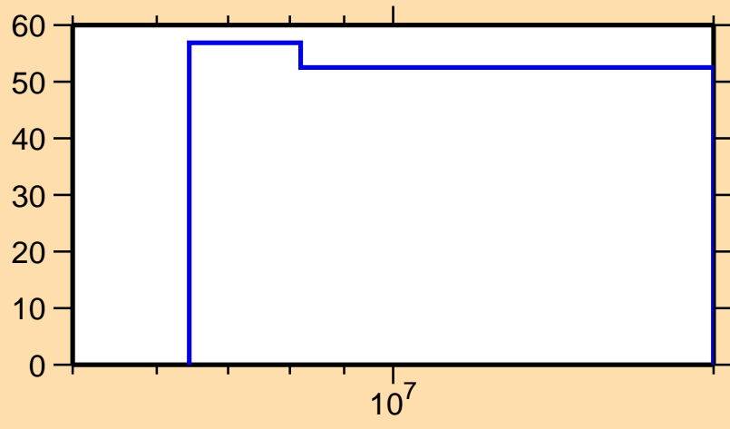
\Delta\sigma/\sigma vs. E for ^{215}\text{Tl}(n,n_1)
