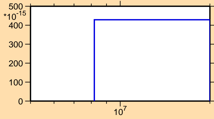
\sigma vs. E for ^{215}\text{Tl} (mt 11)
