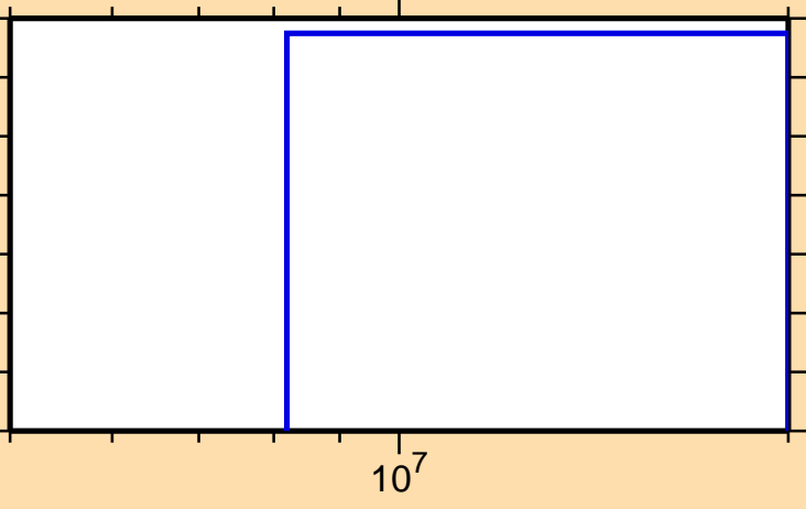
\sigma vs. E for ^{215}\text{Tl}(n,2n\alpha)
