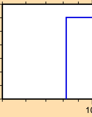
\sigma vs. E for ^{215}\text{Tl} (mt 42)
