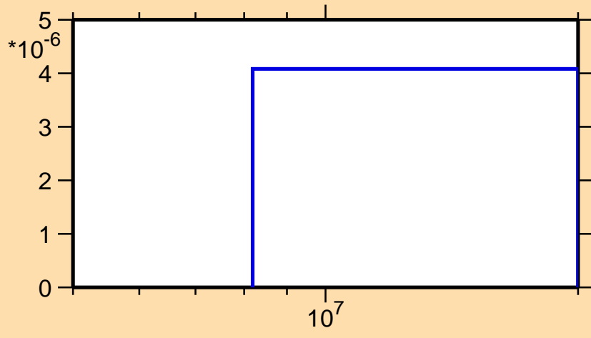
\sigma vs. E for ^{215}\text{Tl}(n,np)
