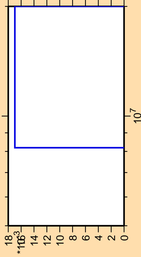
\Delta\sigma/\sigma vs. E for ^{215}\text{Tl} (mt 42)
