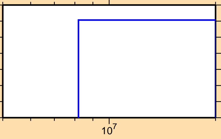
\sigma vs. E for ^{215}\text{Tl}(n,t)
