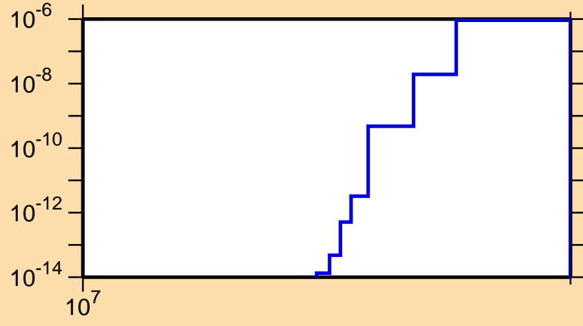
\sigma vs. E for ^{216}\text{Tl}(n,2np)
