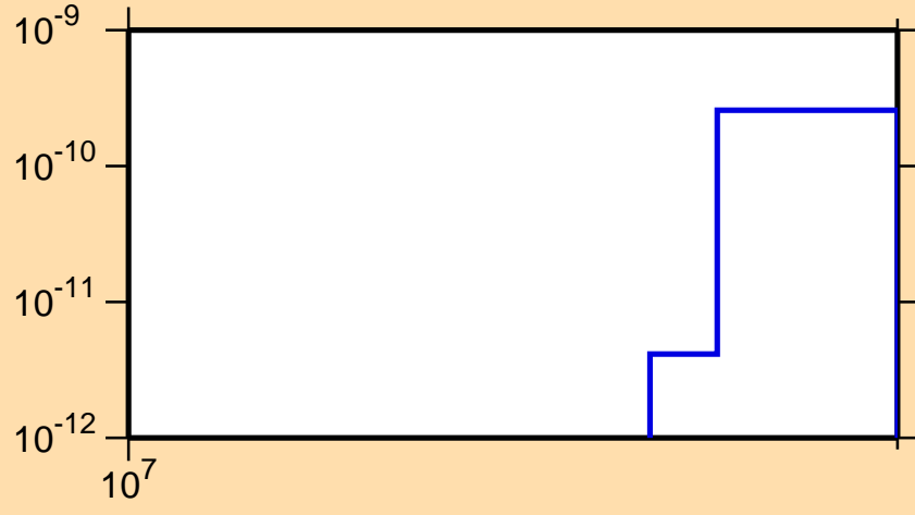
\sigma vs. E for ^{216}\text{Tl}(n,3n\alpha)
