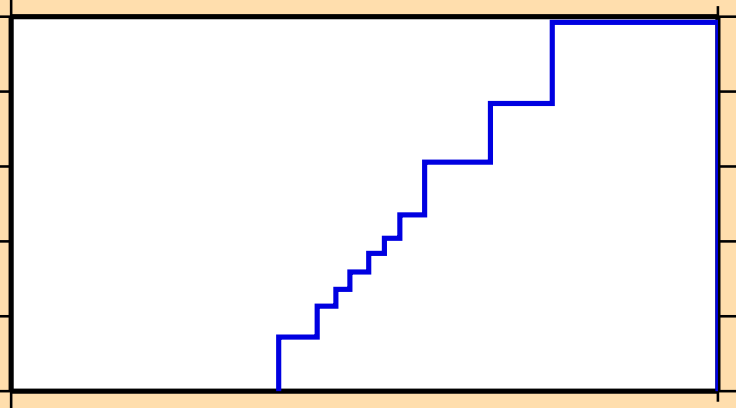
\sigma vs. E for ^{216}\text{Tl}(n,2n\alpha)
