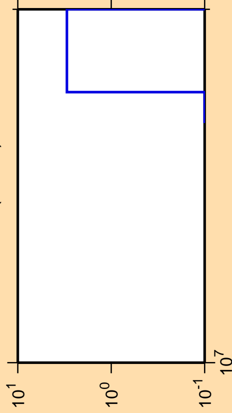
\Delta\sigma/\sigma vs. E for ^{216}\text{Tl} (mt 42)
