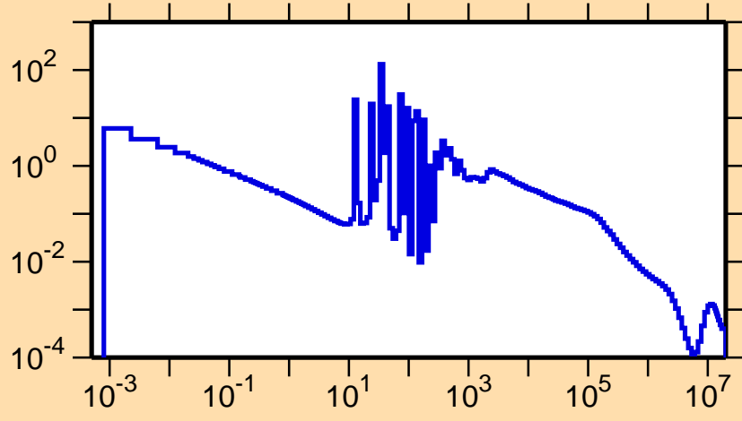
\sigma vs. E for ^{216}\text{Tl}(n,\gamma)
