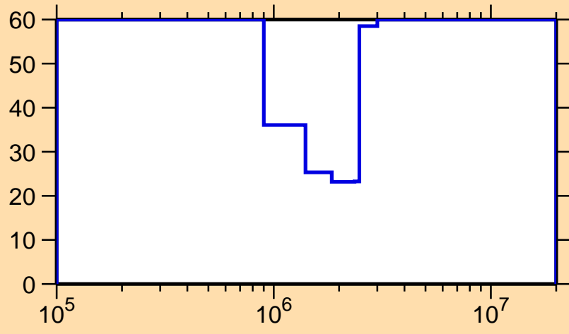
\Delta\sigma/\sigma vs. E for ^{216}\text{Tl}(n,n\text{cont.})
