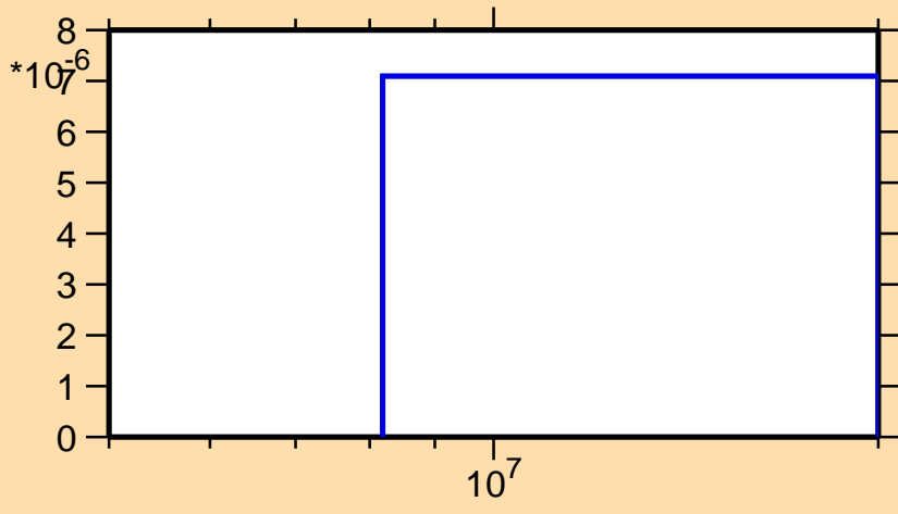
\sigma vs. E for ^{216}\text{Tl}(n,d)
