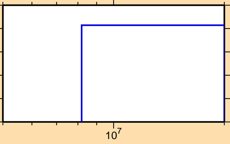
\sigma vs. E for ^{216}\text{Tl}(n,2np)
