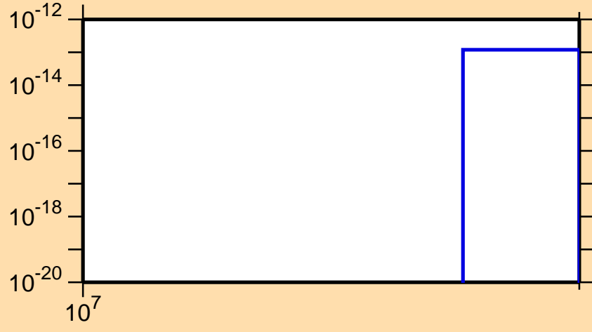
\sigma vs. E for ^{217}\text{Tl} (mt 42)
