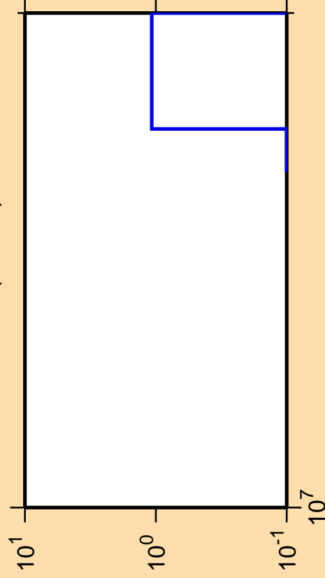
\Delta\sigma/\sigma vs. E for ^{217}\text{Tl} (mt 42)
