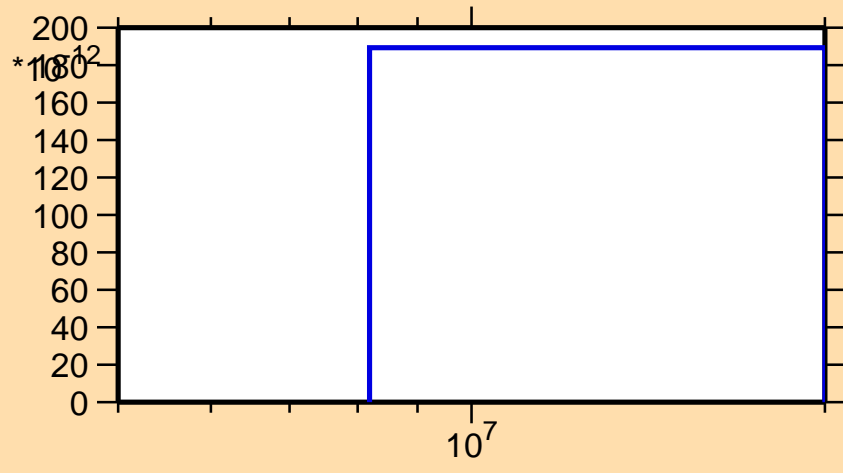
\sigma vs. E for ^{217}\text{Tl}(n,2np)
