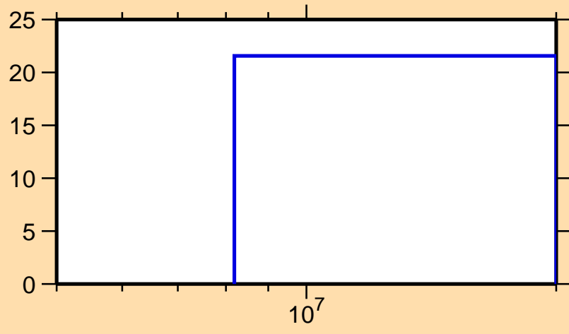
\Delta\sigma/\sigma vs. E for ^{217}\text{Tl}(n,p)
