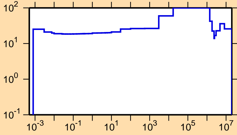
\Delta\sigma/\sigma vs. E for ^{217}\text{Tl}(n,tot.)
