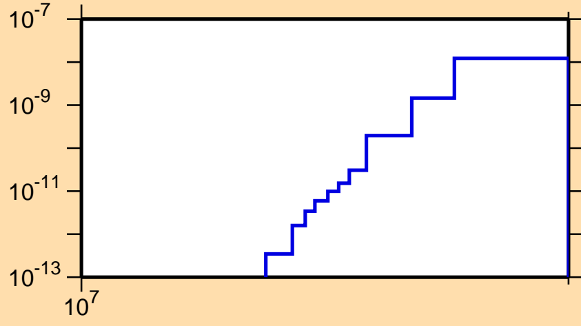
\sigma vs. E for ^{150}\text{Tm} (mt 34)
