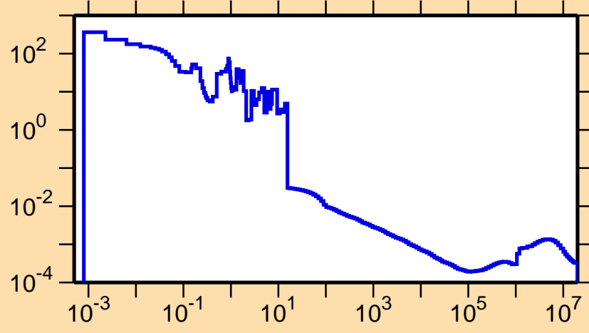
\sigma vs. E for ^{150}\text{Tm}(n,\gamma)
