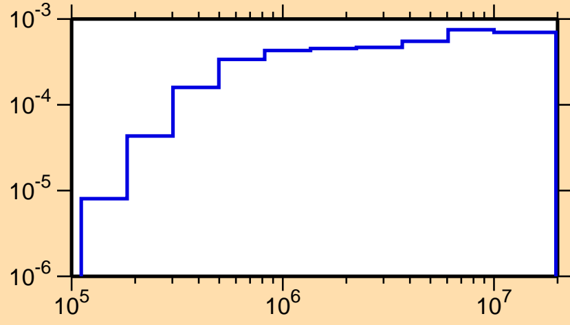
\sigma vs. E for ^{150}\text{Tm}(n,n_2)
