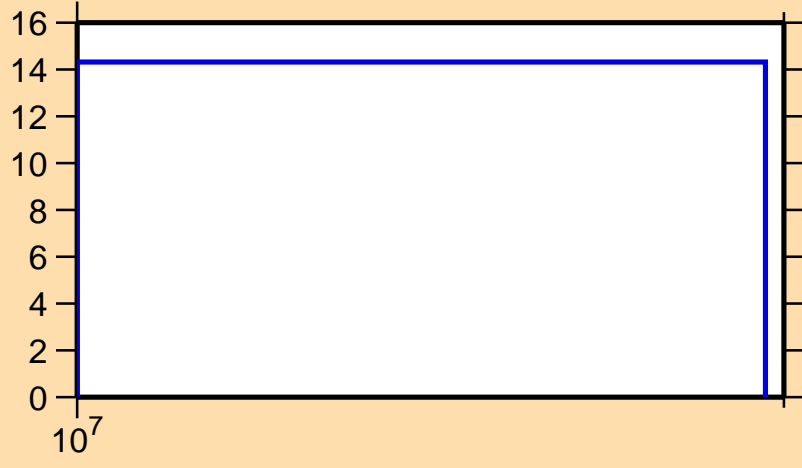
\Delta\sigma/\sigma vs. E for ^{150}\text{Tm}(n,\text{tot.})
