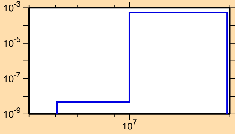
\sigma vs. E for ^{150}\text{Tm}(n,\text{pd})
