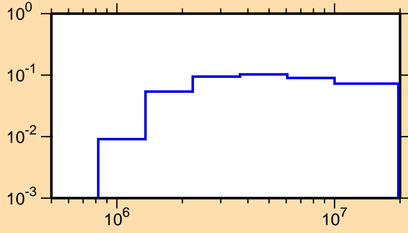
\sigma vs. E for ^{150}\text{Tm}(n,n\text{cont.})
