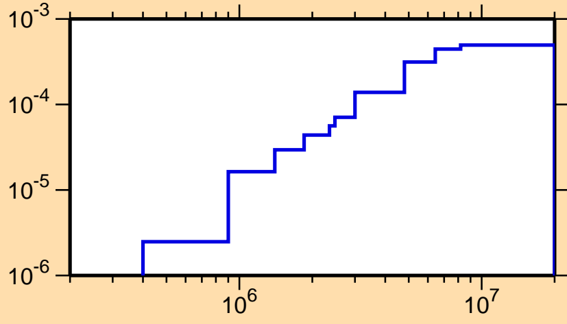
\sigma vs. E for ^{150}\text{Tm}(n,n_4)
