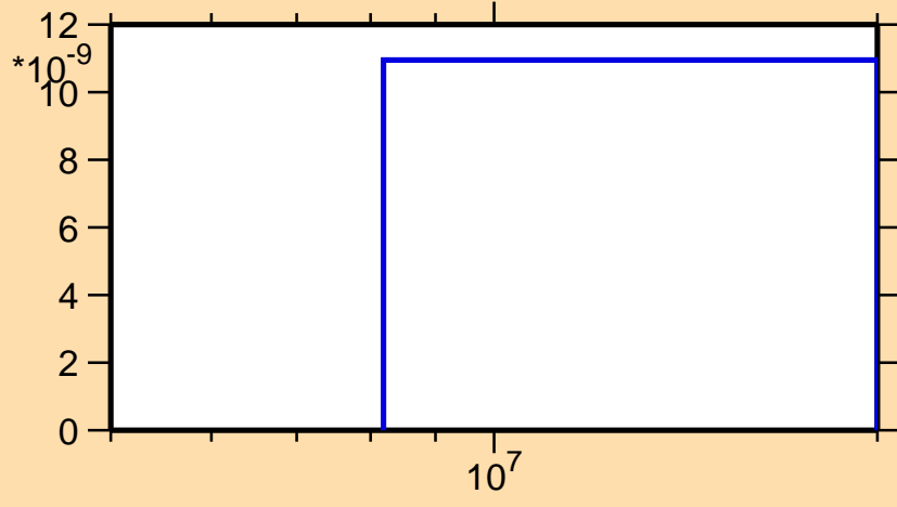
\sigma vs. E for ^{150}\text{Tm}(\text{mt117})
