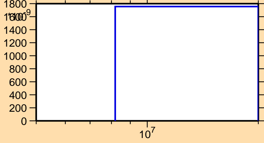
\sigma vs. E for ^{150}\text{Tm}(n,\text{pt})
