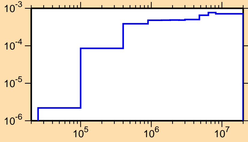
\sigma vs. E for ^{150}\text{Tm}(n,n_1)
