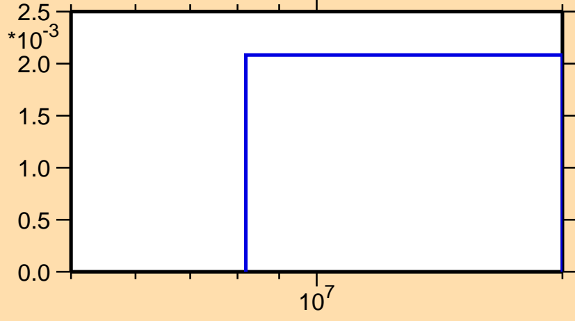
\sigma vs. E for ^{150}\text{Tm}(n,2n)
