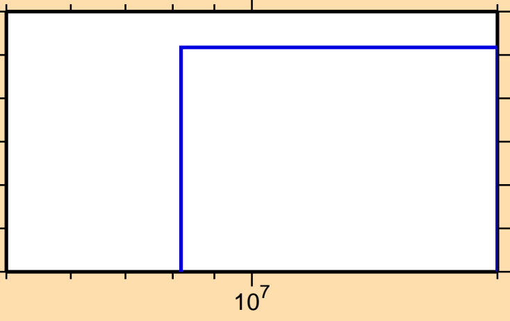
\sigma vs. E for ^{151}\text{Tm}(n,nd)
