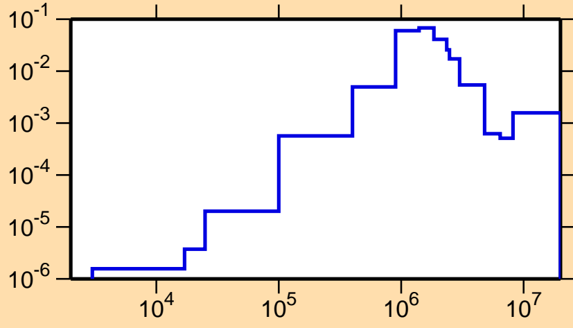
\sigma vs. E for ^{151}\text{Tm}(n,\text{inel.})
