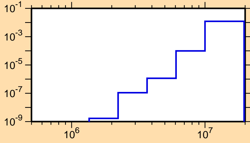
\sigma vs. E for ^{153}\text{Tm}(n,d)
