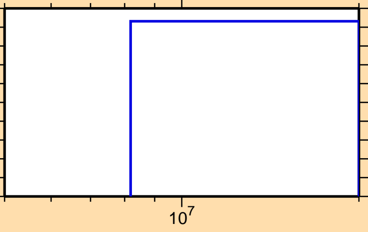
\sigma vs. E for ^{153}\text{Tm}(n,\text{pt})
