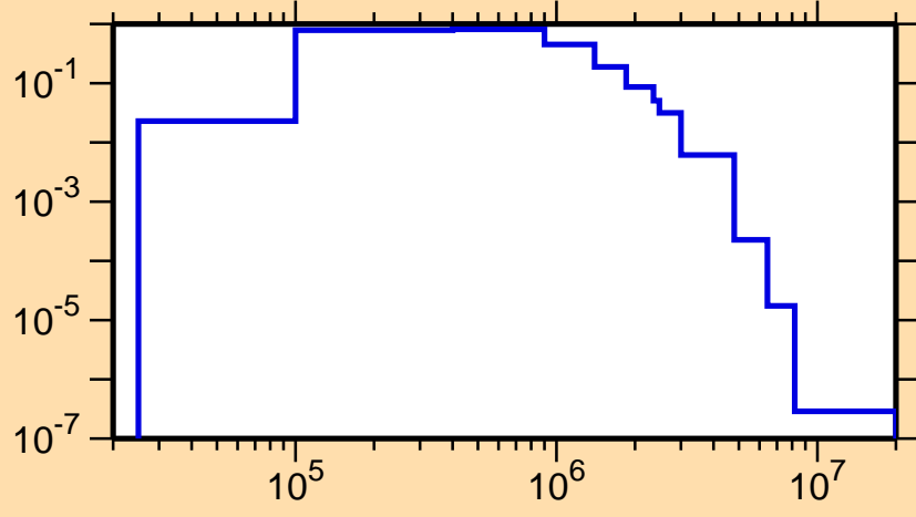
\sigma vs. E for ^{153}\text{Tm}(n,n_2)
