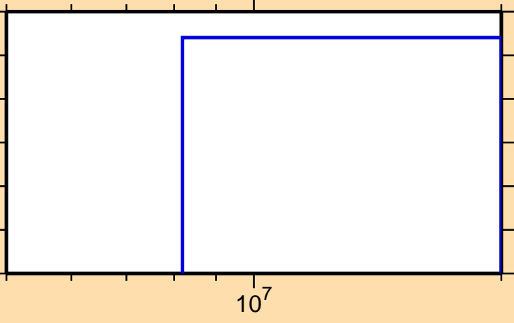
\sigma vs. E for ^{153}\text{Tm}(n,nt)
