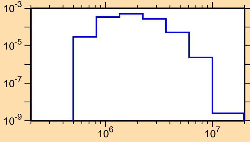
\sigma vs. E for ^{154}\text{Tm}(n,n_4)
