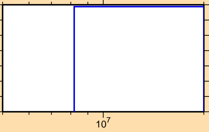
\sigma vs. E for ^{154}\text{Tm}(n,\text{nd})
