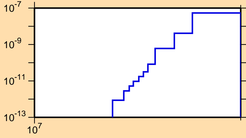
\sigma vs. E for ^{154}\text{Tm} (mt 34)
