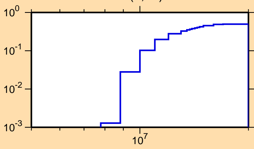
\sigma vs. E for ^{154}\text{Tm}(n,2n)
