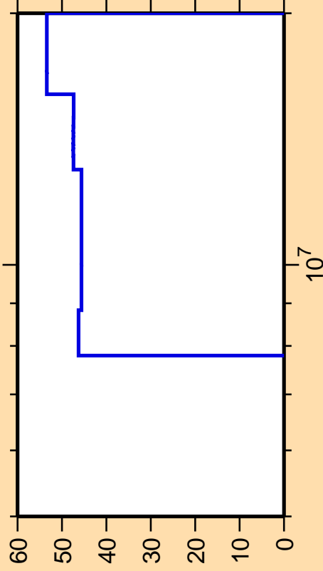
\Delta\sigma/\sigma vs. E for ^{154}\text{Tm}(n,2n)
