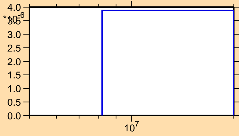
\sigma vs. E for ^{154}\text{Tm}(n,\text{nd})
