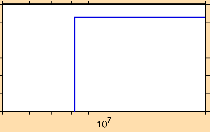
\sigma vs. E for ^{154}\text{Tm}(n,pt)
