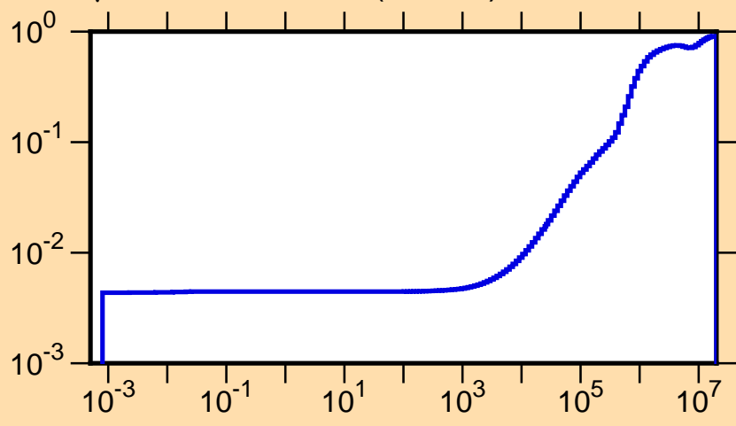
\mu vs. E for ^{155}\text{Tm}(\text{mt251})
