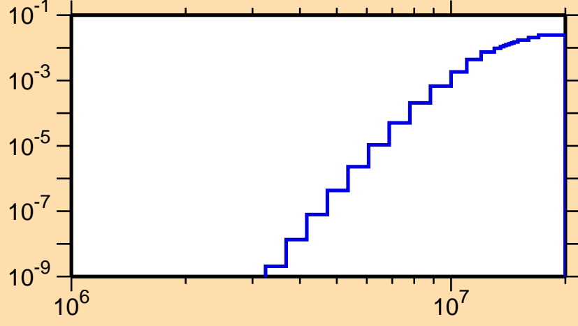
\sigma vs. E for ^{155}\text{Tm}(n,d)
