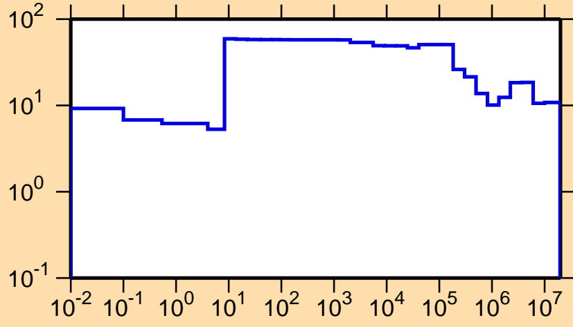
\Delta\sigma/\sigma vs. E for ^{155}\text{Tm}(n,el.)
