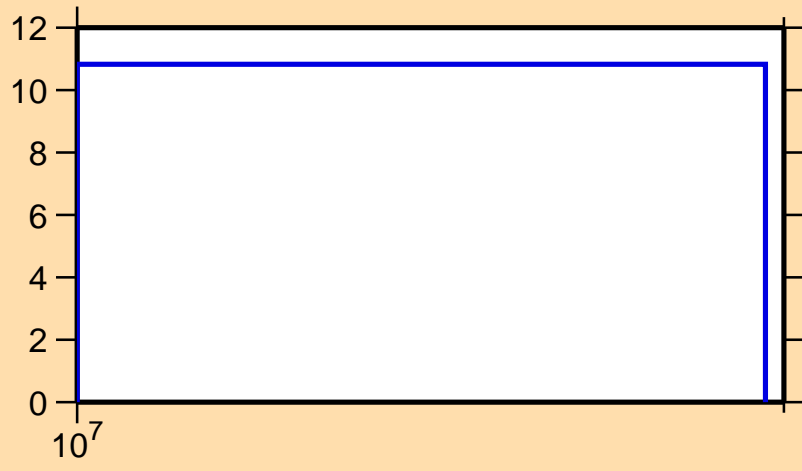
\Delta\sigma/\sigma vs. E for ^{155}\text{Tm}(n,el.)
