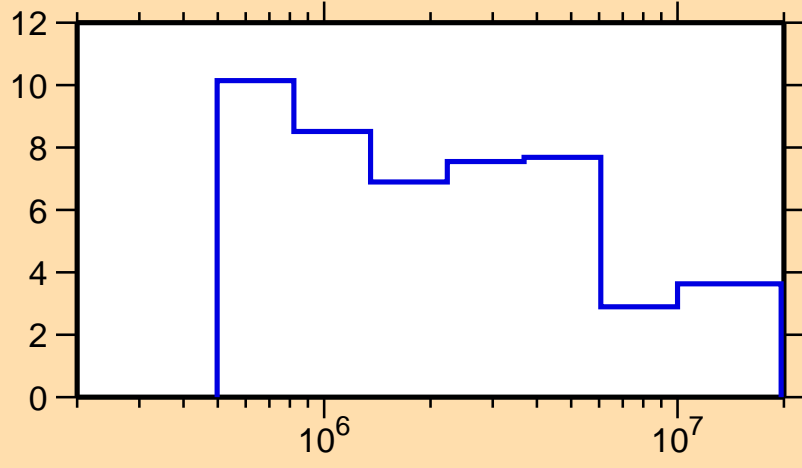
\Delta\sigma/\sigma vs. E for ^{155}\text{Tm}(n, tot.)
