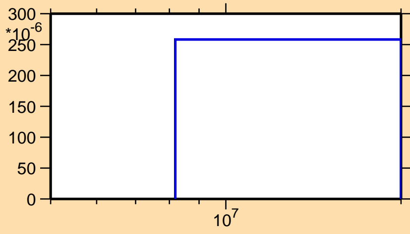
\sigma vs. E for ^{155}\text{Tm}(n,2np)
