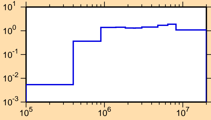
\sigma vs. E for ^{155}\text{Tm}(n,\text{inel.})
