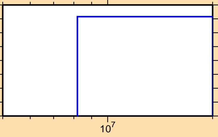
\sigma vs. E for ^{155}\text{Tm} (mt 42)
