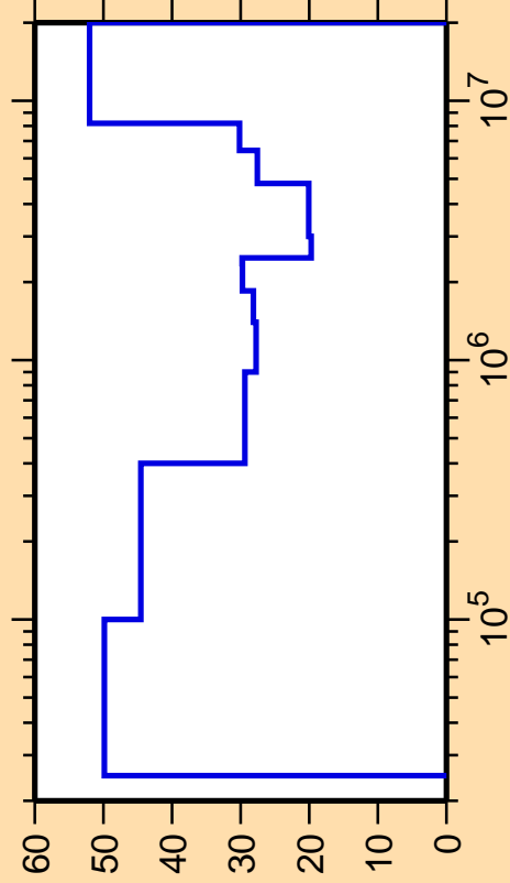
\Delta\sigma/\sigma vs. E for ^{155}\text{Tm}(n,\text{inel.})
