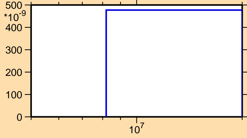
\sigma vs. E for ^{155}\text{Tm}(n,3n)
