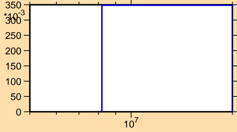
\sigma vs. E for ^{155}\text{Tm}(n,2n)
