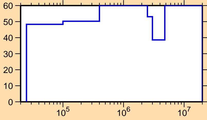
\Delta\sigma/\sigma vs. E for ^{155}\text{Tm}(n,n_1)
