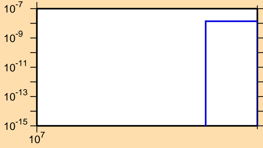
\sigma vs. E for ^{155}\text{Tm}(n,3n\alpha)
