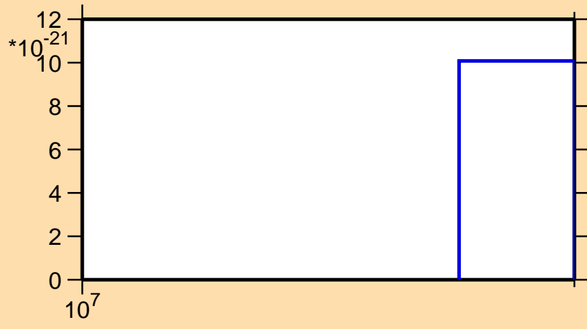
\sigma vs. E for ^{155}\text{Tm} (mt 42)
