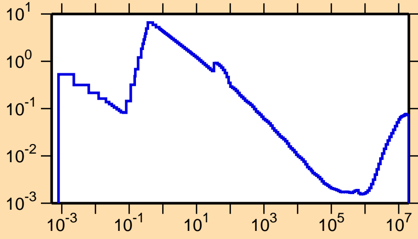
\sigma vs. E for ^{155}\text{Tm}(n,\alpha)
