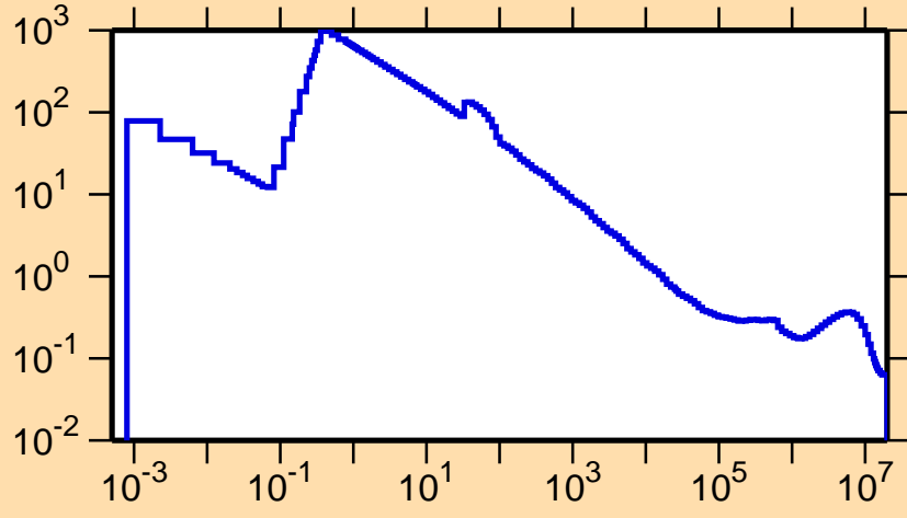
\sigma vs. E for ^{155}\text{Tm}(n,p)
