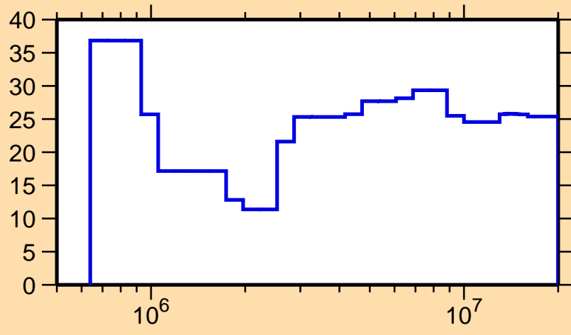
\Delta\sigma/\sigma vs. E for ^{155}\text{Tm}(n,n\text{onel.})
