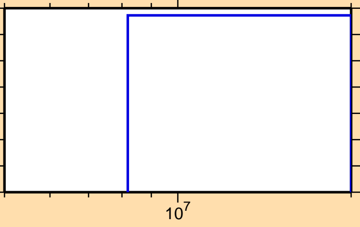
\sigma vs. E for ^{155}\text{Tm}(n,3n)
