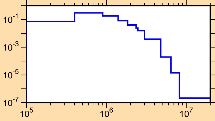
\sigma vs. E for ^{155}\text{Tm}(n,n_3)
