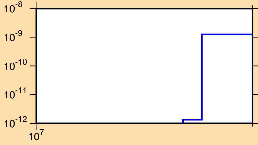
\sigma vs. E for ^{157}\text{Tm}(n,3n\alpha)
