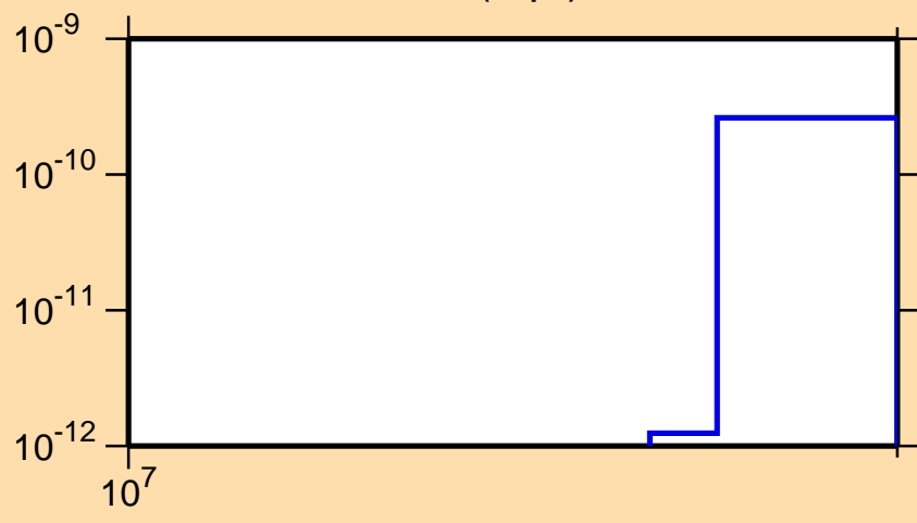
\sigma vs. E for ^{157}\text{Tm}(n,\text{pt})
