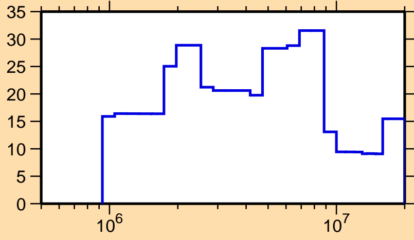
\Delta\sigma/\sigma vs. E for ^{157}\text{Tm}(n, tot.)
