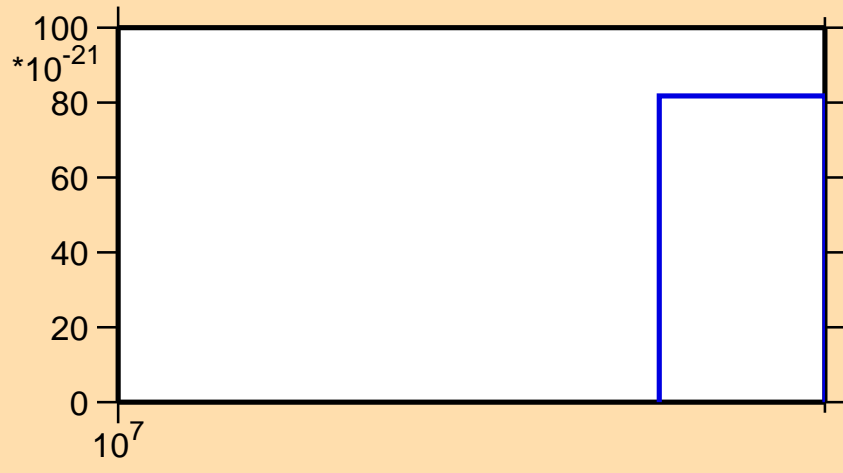
\sigma vs. E for ^{157}\text{Tm} (mt 42)
