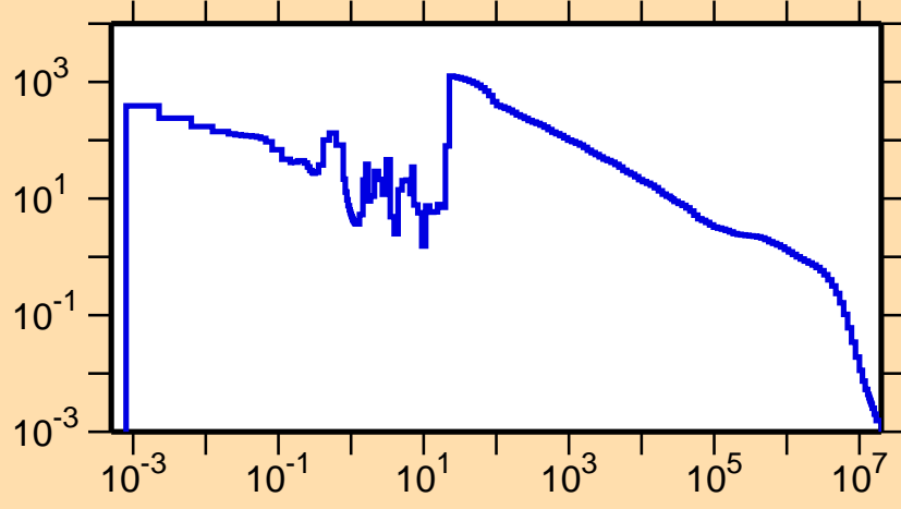
\sigma vs. E for ^{157}\text{Tm}(n,\gamma)
