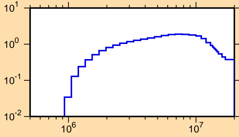
\sigma vs. E for ^{157}\text{Tm}(n,n\text{cont.})
