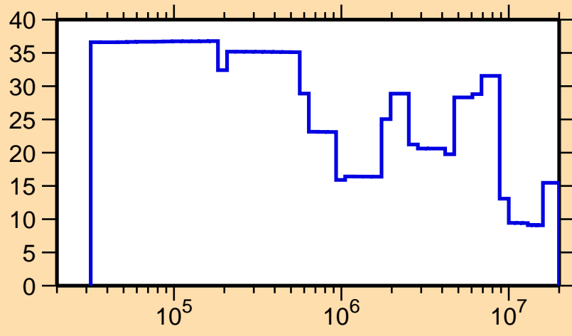
\Delta\sigma/\sigma vs. E for ^{157}\text{Tm}(n,\text{tot.})
