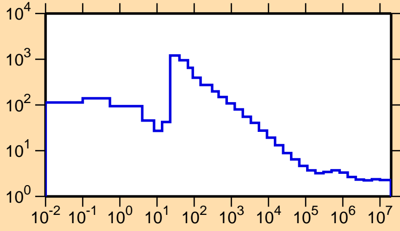
\sigma vs. E for ^{157}\text{Tm}(n,\text{nonel.})
