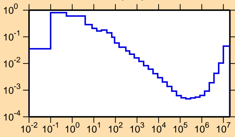
\sigma vs. E for ^{157}\text{Tm}(n,\alpha)
