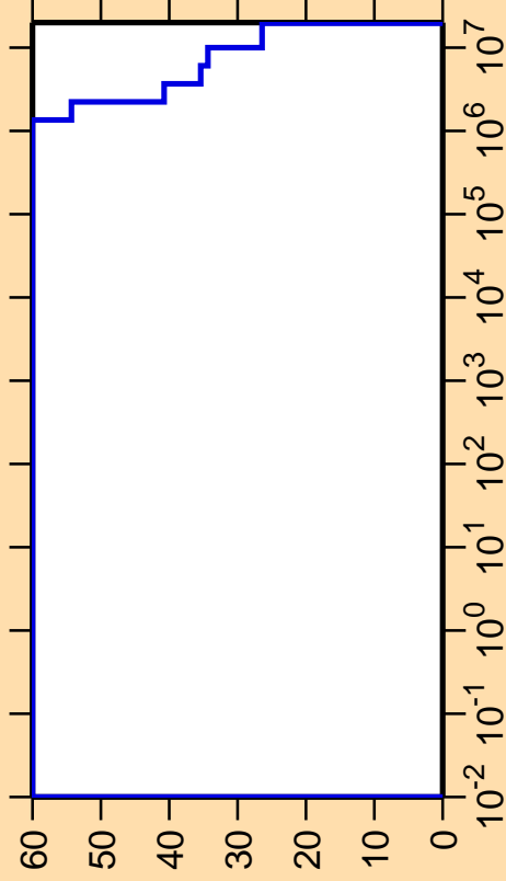
\Delta\sigma/\sigma vs. E for ^{157}\text{Tm}(n,\text{nonel.})
