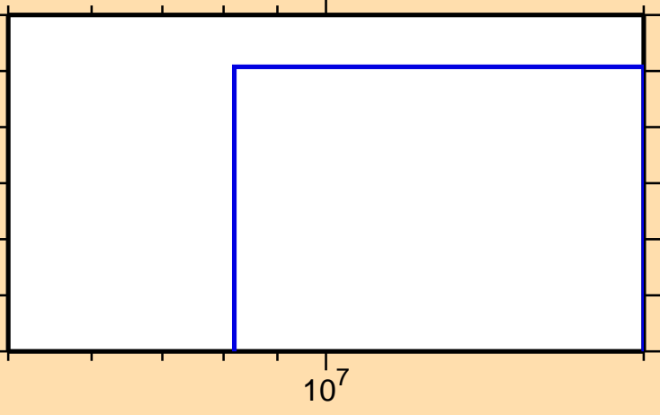
\sigma vs. E for ^{157}\text{Tm}(n,3n)
