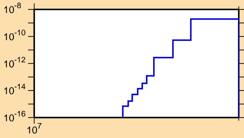
\sigma vs. E for ^{158}\text{Tm} (mt 34)
