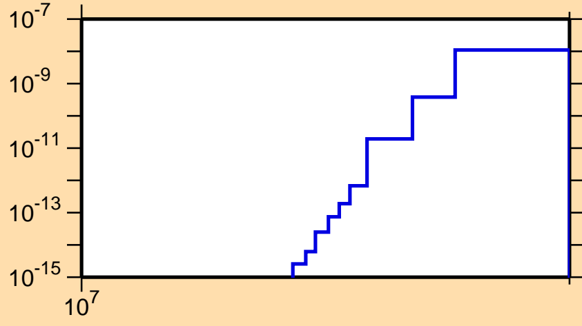
\sigma vs. E for ^{158}\text{Tm}(n,pt)
