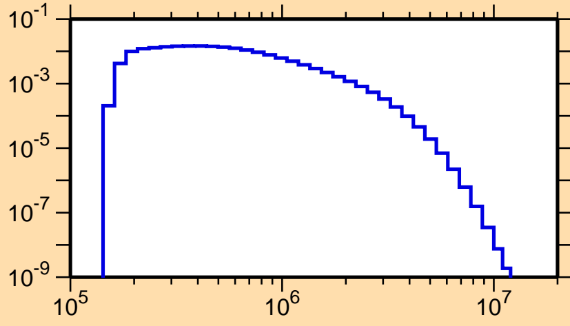
\sigma vs. E for ^{158}\text{Tm}(n,n_3)
