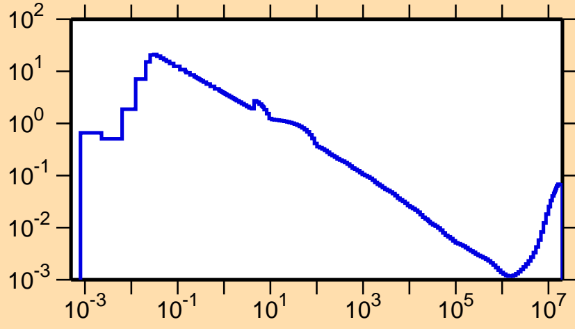
\sigma vs. E for ^{158}\text{Tm}(n,\alpha)
