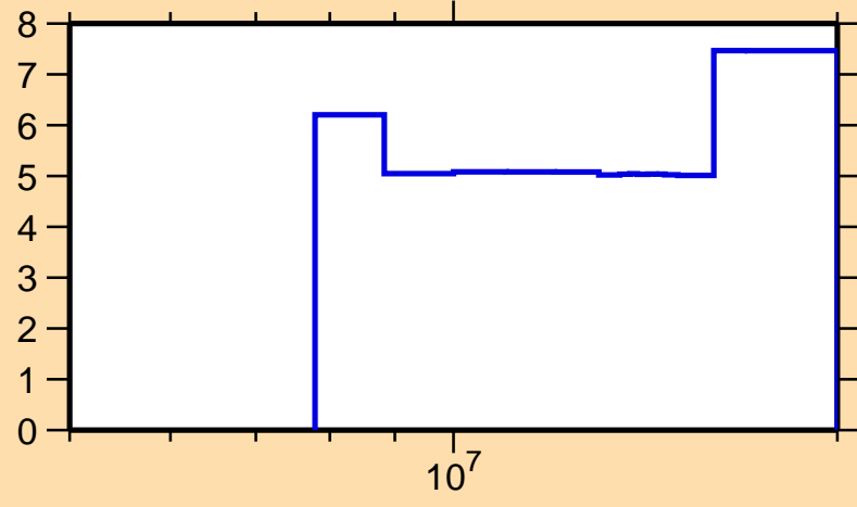
\Delta\sigma/\sigma vs. E for ^{158}\text{Tm}(n,\text{el.})
