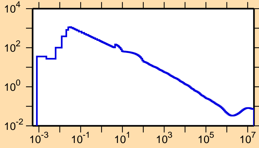
\sigma vs. E for ^{158}\text{Tm}(n,p)
