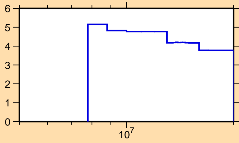
\Delta\sigma/\sigma vs. E for ^{158}\text{Tm}(n,\text{nonel.})
