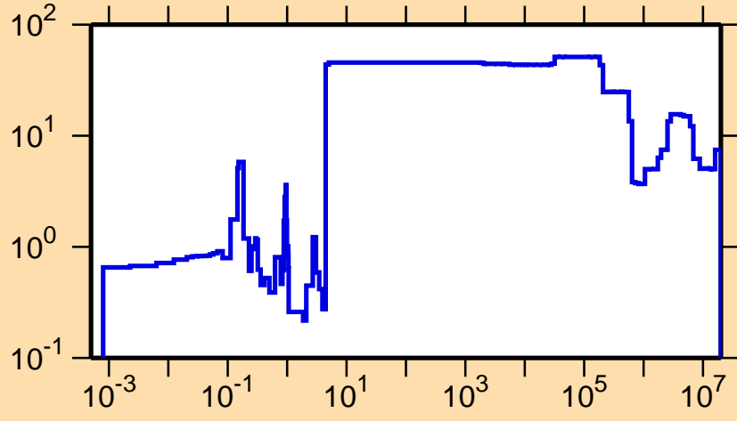
\Delta\sigma/\sigma vs. E for ^{158}\text{Tm}(n,el.)
