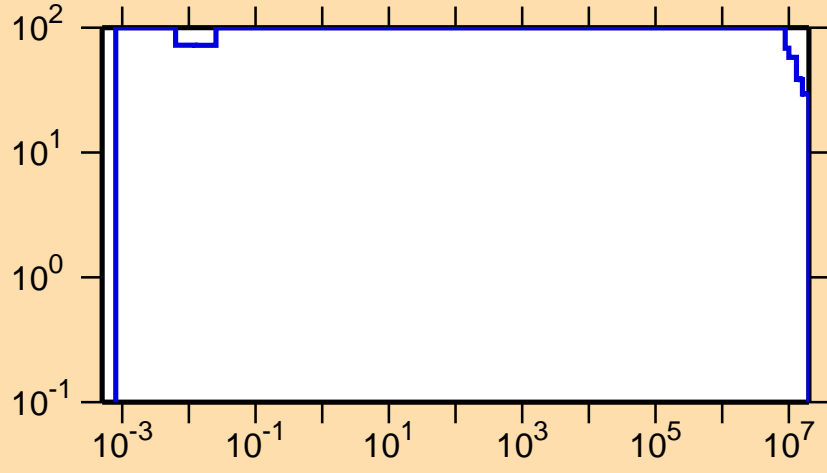
\Delta\sigma/\sigma vs. E for ^{158}\text{Tm}(n,p)
