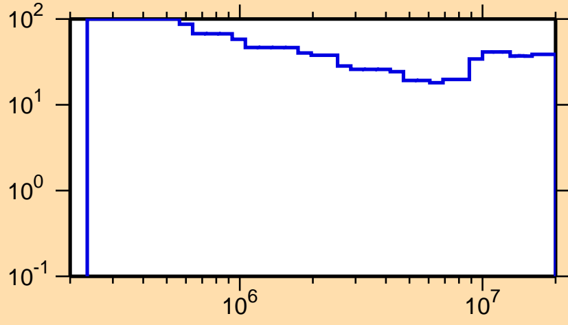
\Delta\sigma/\sigma vs. E for ^{158}\text{Tm}(n,n\text{cont.})
