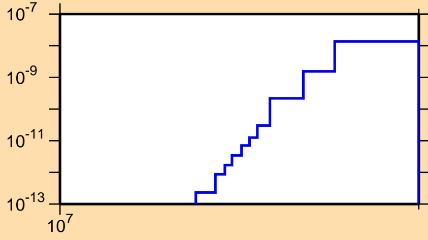
\sigma vs. E for ^{158}\text{Tm}(n,\text{pd})
