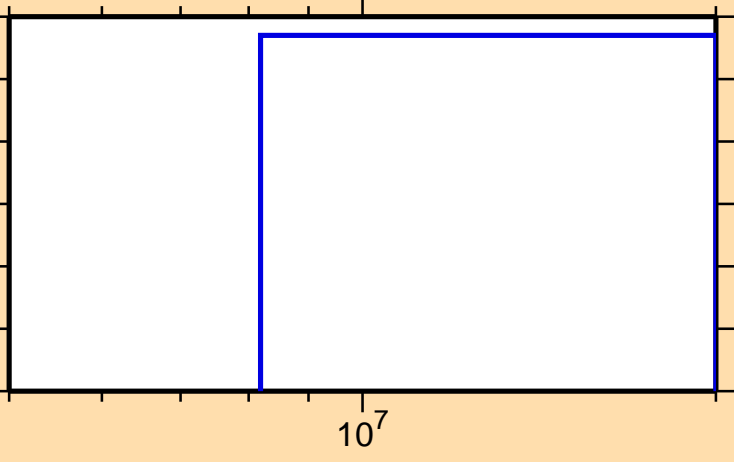
\sigma vs. E for ^{158}\text{Tm}(n,nt)
