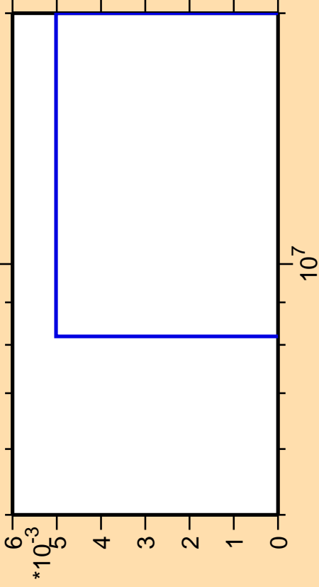
\Delta\sigma/\sigma vs. E for ^{158}\text{Tm}(n,3n\alpha)
