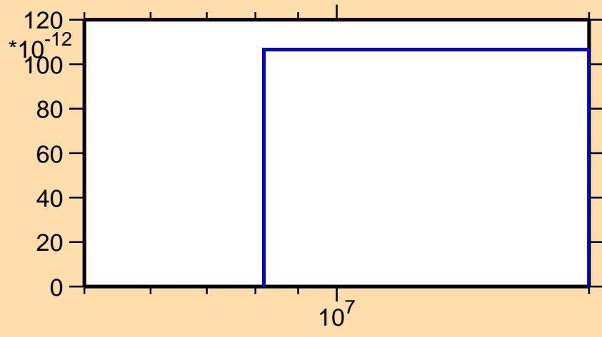
\sigma vs. E for ^{158}\text{Tm}(n,\text{pt})
