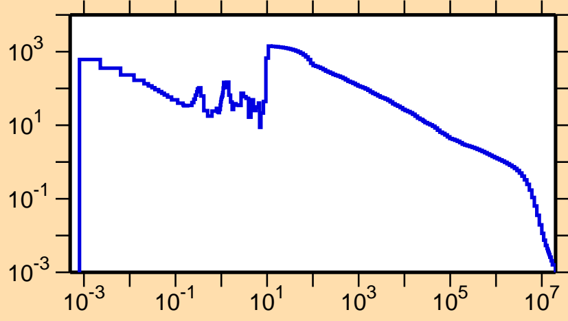
\sigma vs. E for ^{159}\text{Tm}(n,\gamma)
