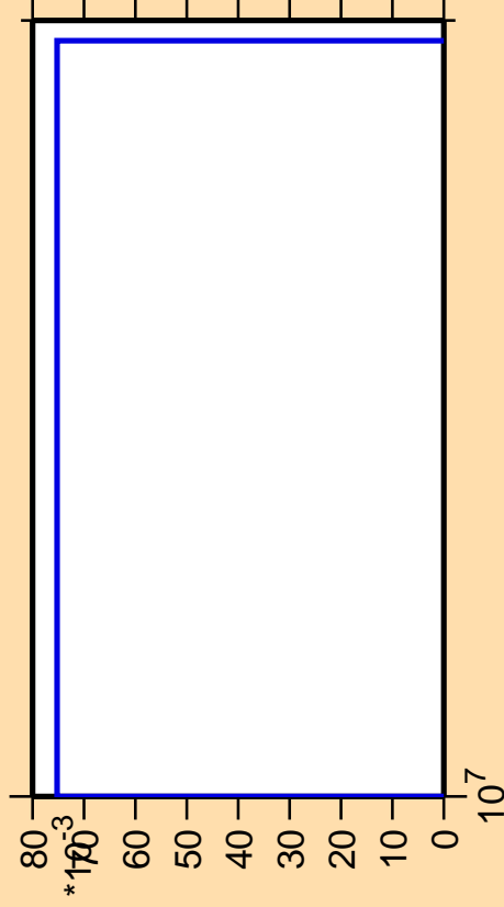
\Delta\sigma/\sigma vs. E for ^{159}\text{Tm}(n,\text{pt})
