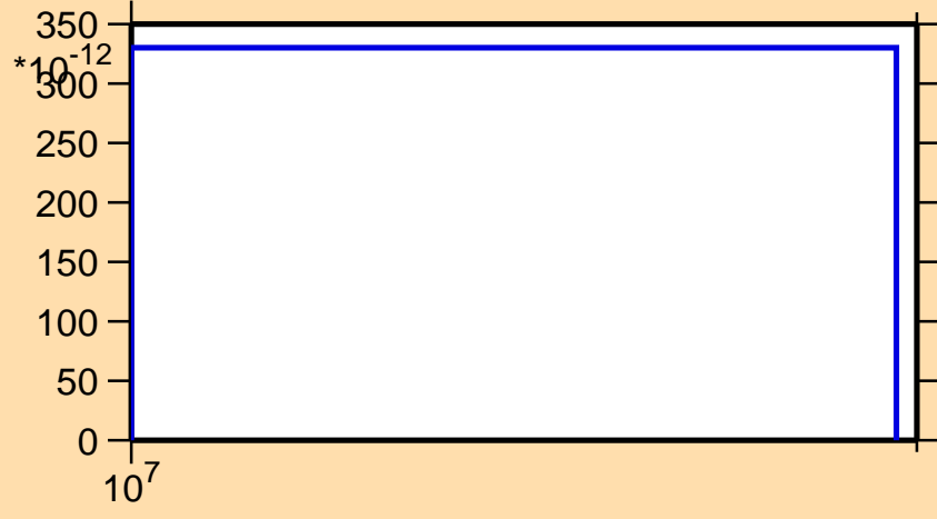
\sigma vs. E for ^{159}\text{Tm}(n,\text{pd})
