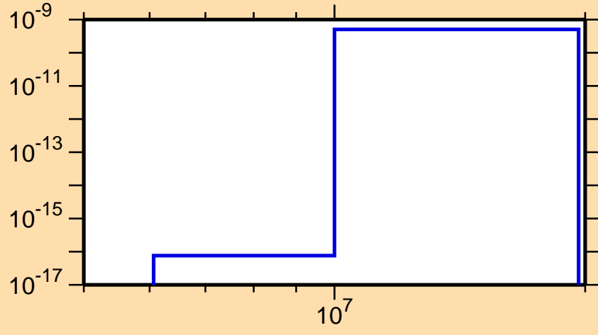
\sigma vs. E for ^{159}\text{Tm}(\text{mt117})
