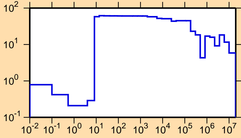
\Delta\sigma/\sigma vs. E for ^{159}\text{Tm}(n,el.)
