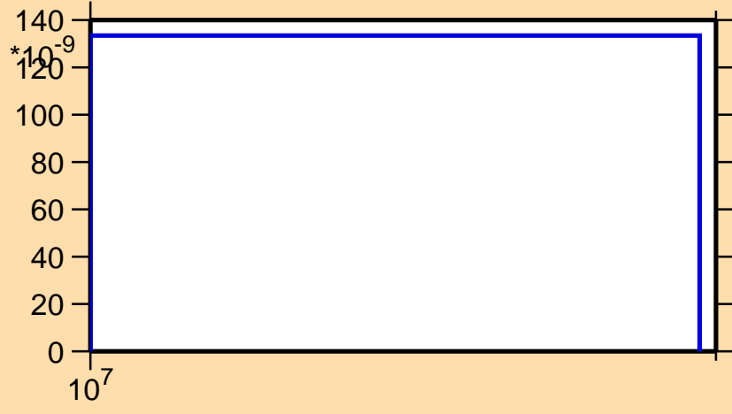
\sigma vs. E for ^{159}\text{Tm}(n,2n\alpha)
