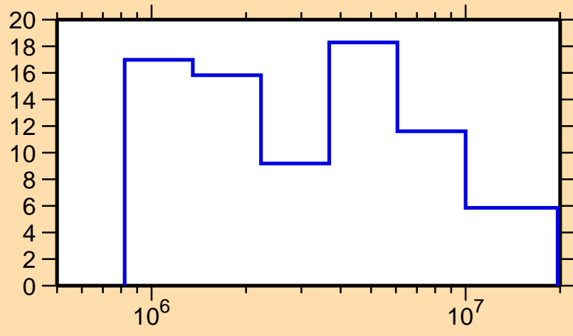
\Delta\sigma/\sigma vs. E for ^{159}\text{Tm}(n,\text{el.})
