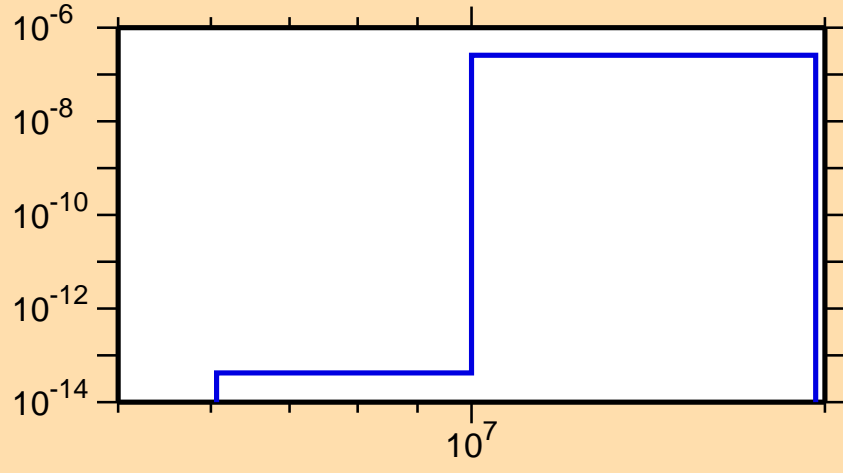
\sigma vs. E for ^{159}\text{Tm}(n,\text{He}3)
