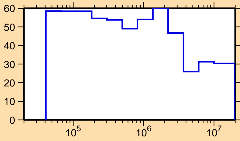
\Delta\sigma/\sigma vs. E for ^{159}\text{Tm}(n,n_1)
